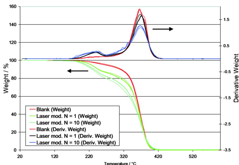
Fig. 3. (Color online) TGA of laser-modified and unmodified PMMA (260 \mu\text{m} initiator-free Vistacryl CQ; \Phi=0.446 \text{ J}/\text{cm}^2 , \Lambda=10 \mu\text{m} , N=1, 10 ).
