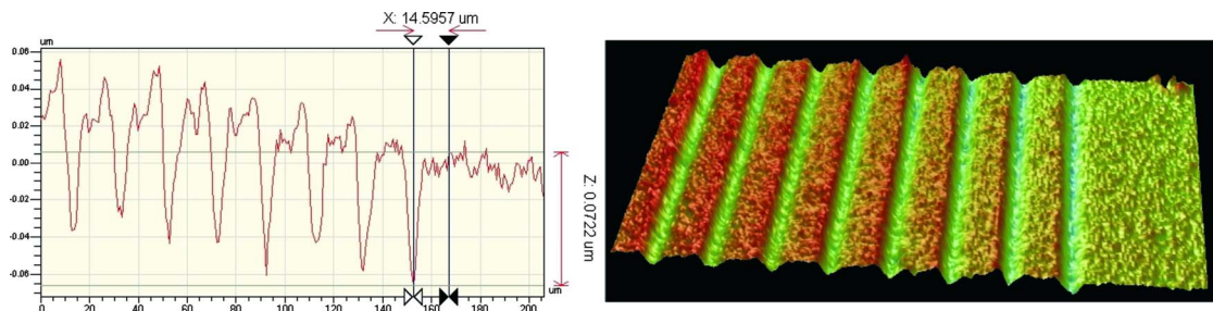
Fig. 4. (Color online) Surface profile of a previously sub-surface grating after etching in MIBK (0.5 mm Vistacryl CQ, \Phi=0.446 \text{ J}/\text{cm}^2 , \Lambda=20 \mu\text{m} , N=1 ).
