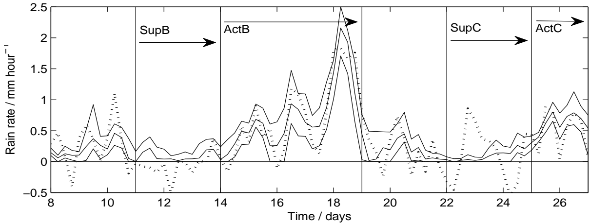
Figure 1: 6-hourly means of the 5th, 50th and 95th percentiles of rainfall rate from an ensemble of SCM runs using the default UM configuration (solid lines), and a budget-derived estimate for the TOGA-COARE IFA (dotted line). This estimate has some negative values, since the observations were insufficient to derive an accurate moisture budget (Petch et al. 2007). The time axis is labelled in whole days since the start of the month of January 1993, as in later figures. Annotations are explained in the text.
