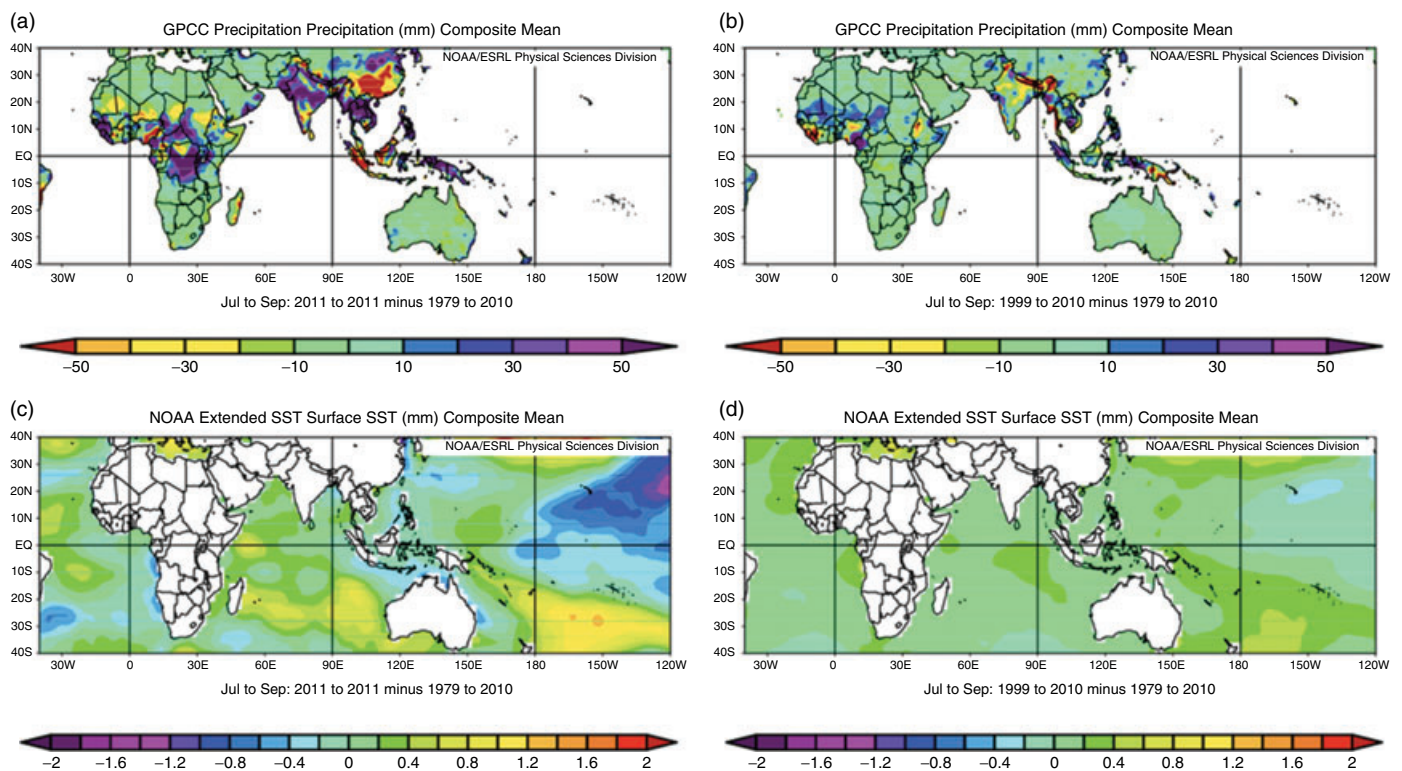
Figure 10. (a) Seasonal precipitation anomalies (mm) for July to September 2011 GPCCC dataset derived from the reference period 1979–2010. (b) As in (a) but for anomalies averaged over 1999–2010. (c) and (d) As in (a) and (b) respectively but for SST.
