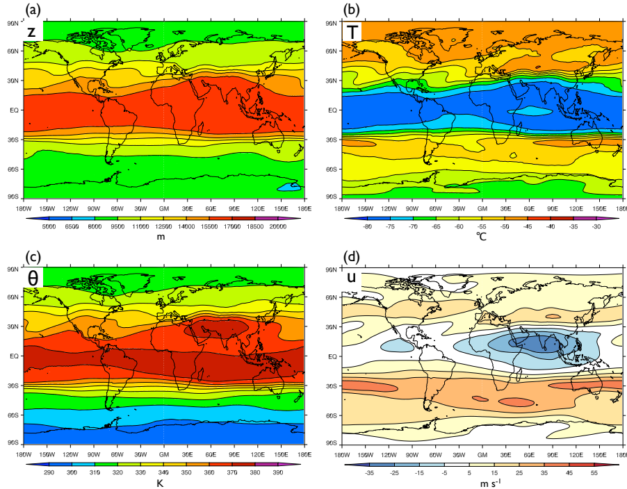
Figure 6: JJA climatologies at the blended tropopause from ERA-Interim (1989-2007). (a): Tropopause height (m) (b): Tropopause temperature (°C) (c): Tropopause potential temperature (K) (d): Tropopause level zonal wind (m s -1 ).
