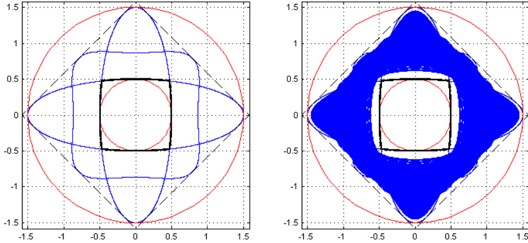
Figure 1: Plots of \text{Spec}(A_c) for the case when c is periodic and \sigma = 0.5 . The two plots show the sets \pi_{N, \sigma} \subset S_\sigma , the union of the spectra for all sequences c of period \leq N , for N = 2 (left) and N = 12 (right). The two ellipses visible in the left-hand plot, the boundaries of E_\sigma and E_{-\sigma} defined in (32) and (33), are the components of \pi_{1, \sigma} ; the other closed curve is \text{Spec}(A_c) for c = \sigma c^{(1, -)} , i.e. c_n = (-1)^n \sigma , given explicitly in Lemma 24. Also shown in each plot are the boundaries of the inclusion sets from Lemma 26, namely the circles of radius 1 \pm \sigma , and, in dashed lines, the boundary of the set (35). The boundary of H_\sigma , which we conjecture is a hole in the spectrum S_\sigma , is highlighted in a thicker line.
