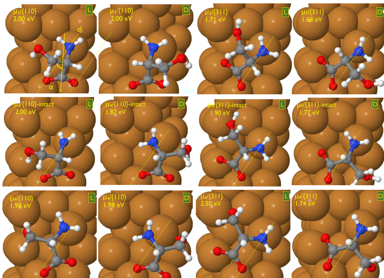
Figure 5: DFT-optimized \mu_3 and \mu_4 adsorption geometries for L- and D-serine on the {110} and {311} microfacets of Cu{531} S ; top to bottom: \mu_3 with intact \beta -OH, \mu_4 with intact \beta -OH, \mu_4 with de-protonated \beta -OH (red=oxygen, blue=nitrogen, gray=carbon, white=hydrogen). The respective adsorption energies are indicated in the Figure; the dotted lines ( 0^\circ ) indicate the [11\bar{2}] crystallographic direction.
