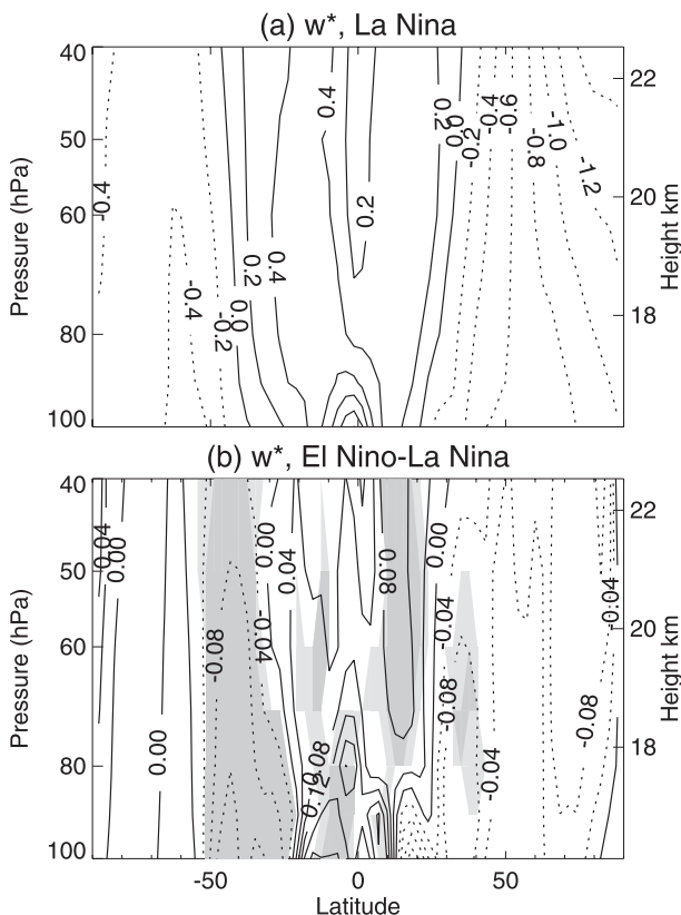
FIG. 3. DJFM zonal mean residual vertical velocity \bar{w}^* for (a) the La Niña simulations ( CI = 0.2 \text{ mm s}^{-1} ) and (b) the difference between El Niño and La Niña ( CI = 0.02 \text{ mm s}^{-1} ). Positive values denote upwelling and light and dark gray regions are significantly different from zero at the 95% and 99% levels, respectively. Dotted contours indicate negative values.
