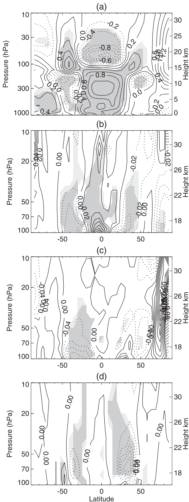
FIG. 6. Difference between El Niño and La Niña composites of the chemistry CMAM 1960–2000 simulations in DJFM. (a) Zonal mean
