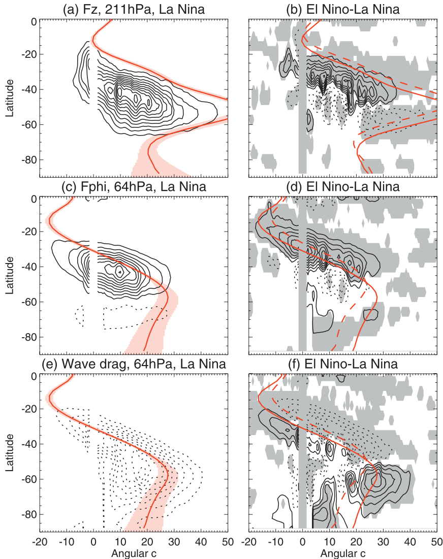
FIG. 7. Cospectra of (top) vertical E-P flux on the 211-hPa level, (middle) meridional E-P flux on the 64-hPa level, and (bottom) wave drag ( \mathbf{V} \cdot \mathbf{F}/\rho a \cos\phi ) on the 64-hPa level. (left) The La Niña climatology and (right) the difference between El Niño and La Niña for the DJFM season. Contour intervals are as follows: (a) 1 \times 10^3 \text{ kg s}^{-2} \Delta c^{-1} , (b) 5 \times 10^2 \text{ kg s}^{-2} \Delta c^{-1} , (c) 1 \times 10^4 \text{ m}^3 \text{ s}^{-2} \Delta c^{-1} , (d) 5 \times 10^3 \text{ m}^3 \text{ s}^{-2} \Delta c^{-1} , (e) 5 \times 10^{-3} \text{ m s}^{-1} \text{ day}^{-1} \Delta c^{-1} , and (f) 2.5 \times 10^{-3} \text{ m s}^{-1} \text{ day}^{-1} \Delta c^{-1} , where \Delta c is 0.5 \text{ m s}^{-1} . The solid red line shows the La Niña \bar{u}/\cos\phi and the dashed line shows the El Niño \bar{u}/\cos\phi . For the La Niña climatology plots, the red shading indicates \pm 1 standard deviation about the mean in \bar{u}/\cos\phi . For the difference plots, gray regions are statistically significant at the 95% level. Dotted contours indicate negative values.
