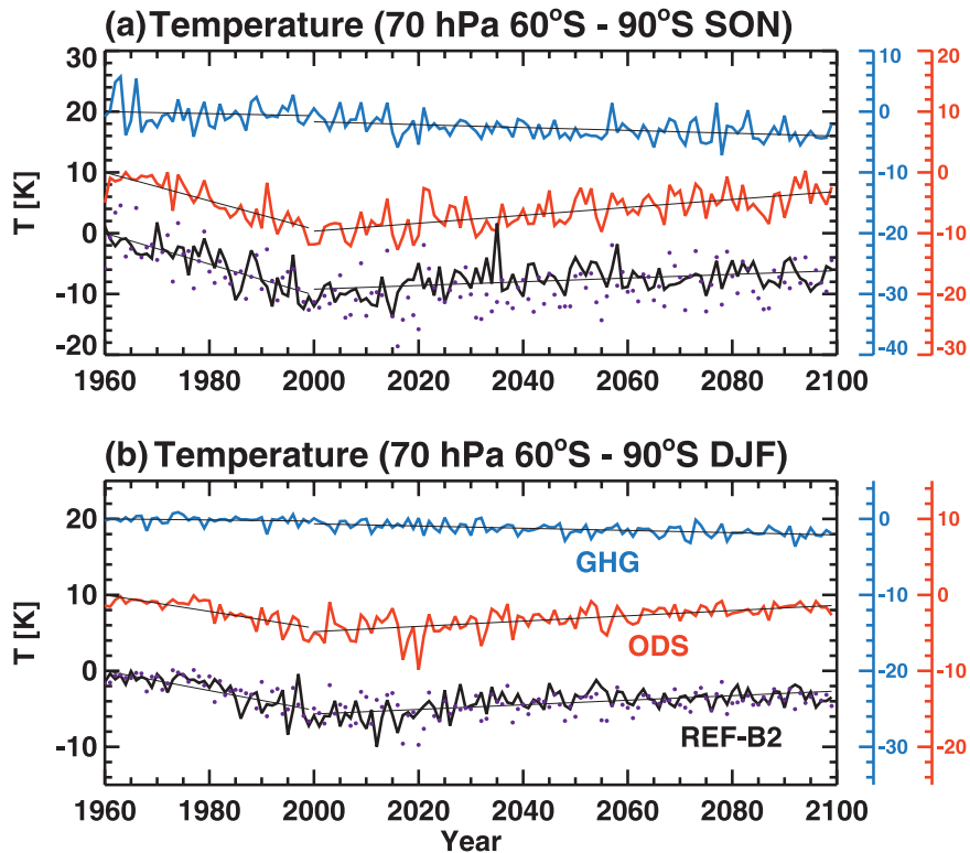
FIG. 2. Time series of polar cap average ( 60^{\circ} – 90^{\circ} S) temperature anomalies at 70 hPa for SH (a) spring (SON) and (b) summer (DJF): GHG (blue), ODS (red), and REF-B2 (black) simulations, and the sum of the GHG and ODS simulations (purple dots). For clarity the red and blue curves are shifted with respect to the black; their color-coded axes are given on the right. The straight lines are linear fits computed from 1960–99 and 2000–99. Ensemble averages are shown. Anomalies are computed with respect to the 1960 baselines given by the intercepts of the linear fits computed from 1960–99 (see text). The actual temperature time series can be recovered by adding the anomaly time series to the 1960 baselines, which for the REF-B2, GHG, and ODS simulations are, respectively, 206.9, 204.8, and 206.8 K for SON and 232.3, 231.2, and 232.2 for DJF.
