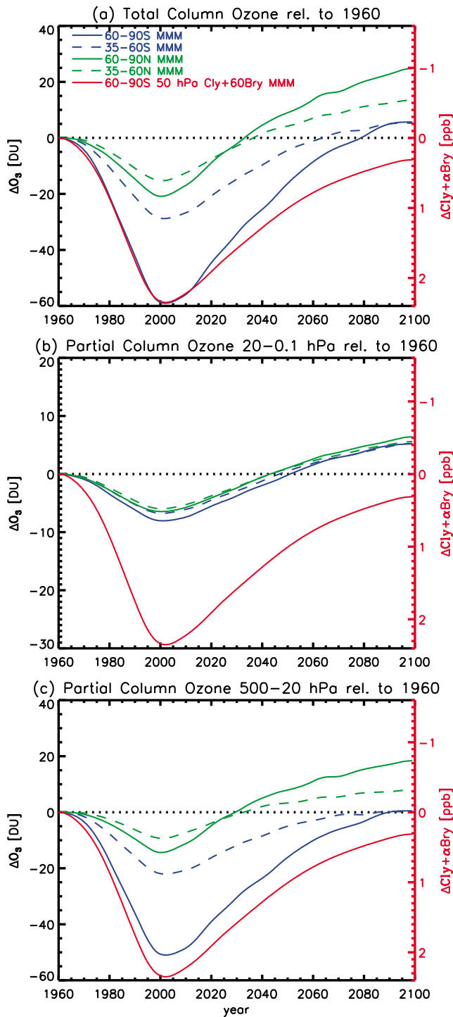
Figure 10. MMM of (a) total and (b and c) partial column ozone amounts for middle (35°–60°S and 35°–60°N; dashed curves) and high (60°–90°S and 60°–90°N; solid curves) latitudes and Cl + \alpha Br for high latitudes (60°–90°S) for reference.
