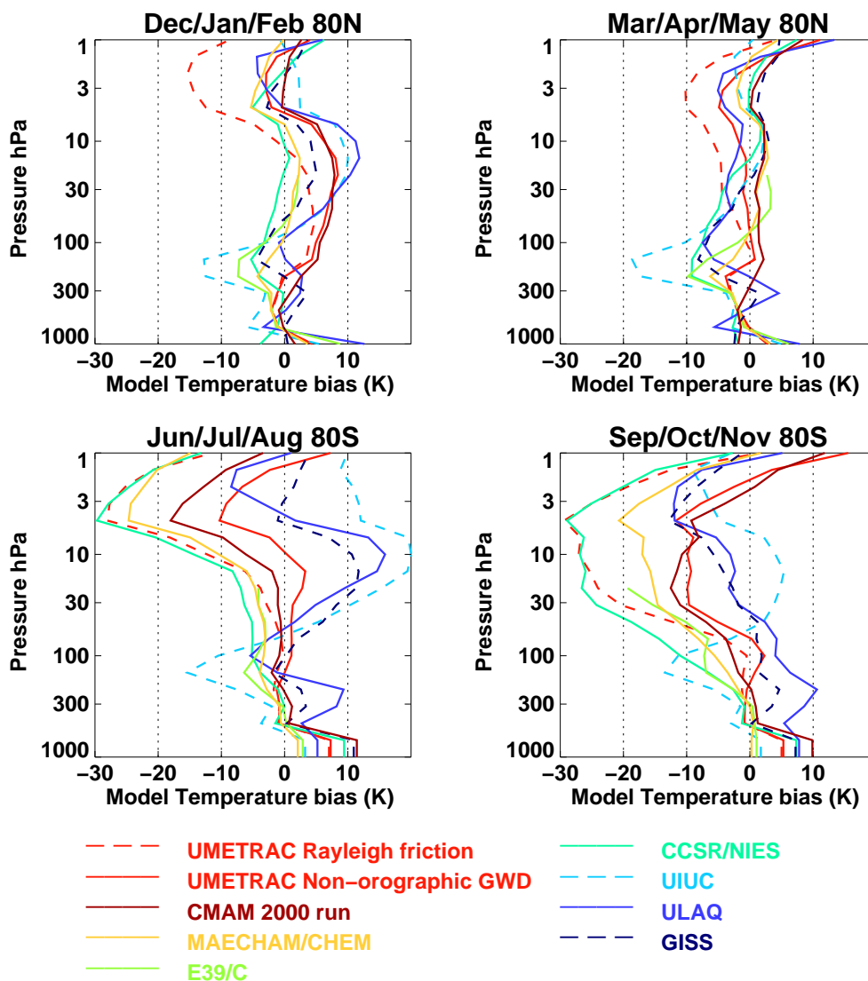
Fig. 3. Temperature biases at 80^{\circ} N and 80^{\circ} S for the winter and spring seasons, as a function of pressure. To determine the bias, a climatology determined from 10 years of UKMO data assimilation temperatures was subtracted from the model results averaged for the same years as indicated in Fig. 1.
