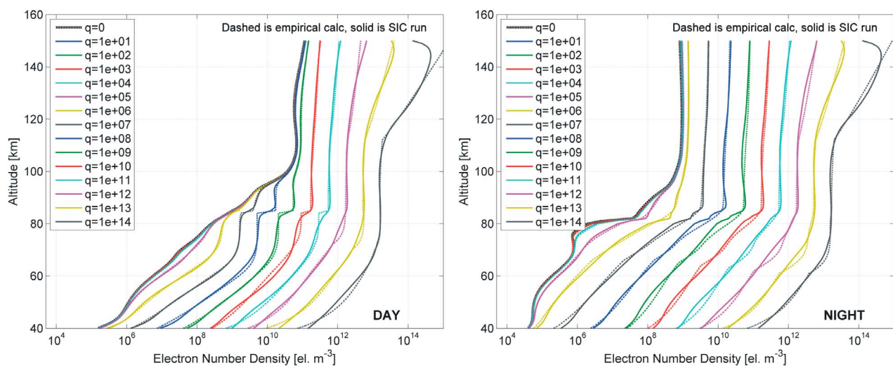
Figure 3. Electron number density calculations undertaken for ionization rates ( q [electrons m^{-3} ]) which were constant with altitude for (left) day and (right) night conditions. The solid curves are the results from the Sodankylä Ion and Neutral Chemistry (SIC) model, while the dashed curves are from an equilibrium electron density model which has been fitted to the SIC results. Note that the curves for q < 10^4 electrons m^{-3} , are almost indistinguishable on this plot from the electron number density for q = 0 .
