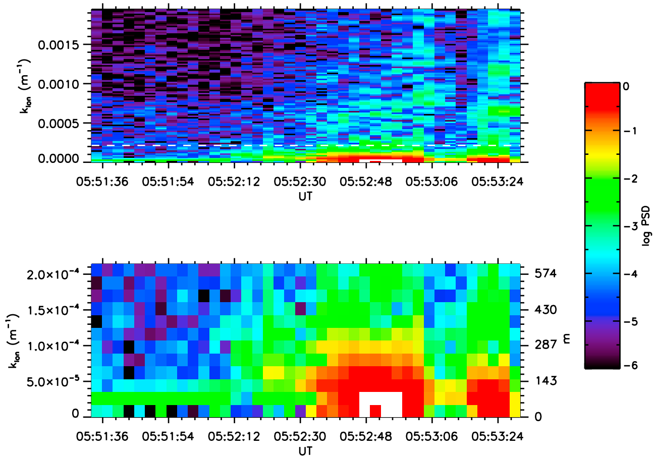
Figure 2. Auroral fluctuations as a function of k_{ion} and time for (a) all azimuthal wave numbers and (b) low wave numbers below the white line shown in Figure 2a. (b) Right-hand axis shows the wave numbers calculated as dimensionless azimuthal wave number, m .
