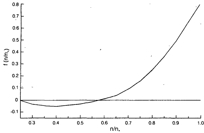
FIG. 12. Dissipative function in Eq. (19).
