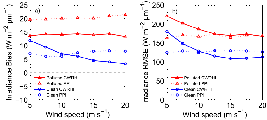
Figure 8. Effect of wind speed on (a) bias and (b) RMSE of surface downwelling irradiance ( W m^{-2} \mu m^{-1} ) at 870 nm for the clean and polluted cases, based on CWRHI and PPI scans with radar sensitivity -37.5 dBZ and solar zenith angle is 45^\circ .
