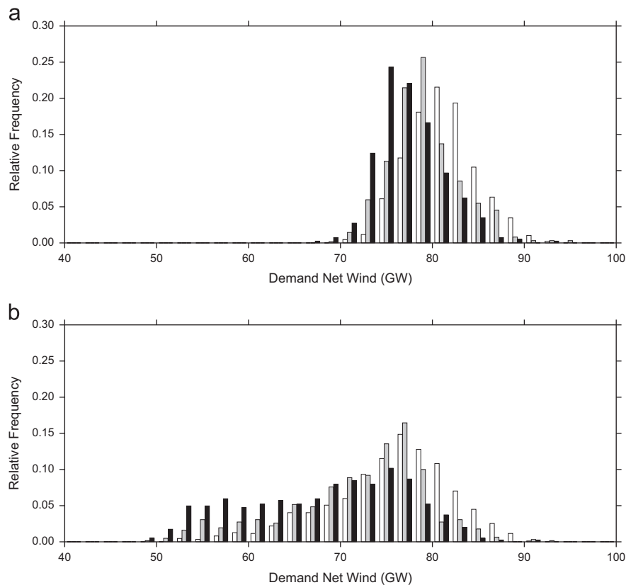
Fig. 5. Probability distribution of daily demand-net-wind (DNW) for March 1950–2010 composited by NAO state; negative (white), neutral (grey) and positive (black). Wind-power capacity levels representative of (a) 2010 and (b) 2020, assuming no change in demand behaviour (scenarios 2010c and 2020 in Table 5). Wind and demand are modelled as described in Section 2.
