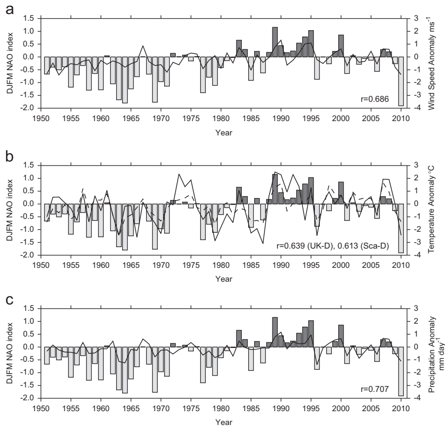
Fig. 3. Time series of the DJFM NAO index (bars) plotted against the DJFM anomalies (from the 1981 to 2010 climatology) of wind speed, temperature, and precipitation rate over the study regions. (a) Wind speed anomalies in UK-S region; (b) temperature anomalies in Sca-D (solid line) and UK-D (dashed line) regions; (c) precipitation anomalies in Nor-S region. The Pearson linear correlation coefficient, denoted by r , is also shown.
