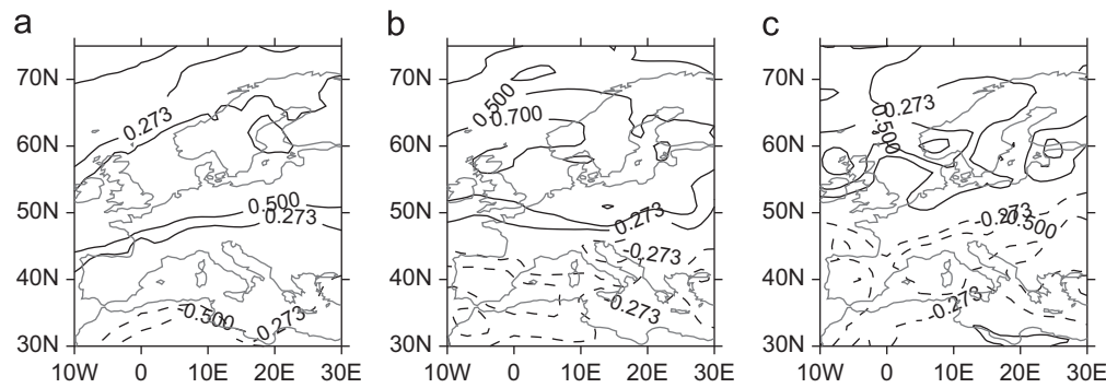
Fig. 1. Climatic impacts of the NAO in winter, given as the 1950–2010 temporal correlation between the DJFM NAO index and the DJFM average of a) 2m temperature T ( ^{\circ}\text{C} ); b) 10m wind speed u ( \text{ms}^{-1} ); c) precipitation rate Q ( \text{mm day}^{-1} ). Seasonal averages of T , u and Q are computed from the NCEP reanalysis data introduced in Section 2. The 0.273 contour would indicate the boundary of statistical significance at the 95% confidence level under the assumption of Gaussian variables. Here and throughout the study Pearson linear correlations are used.
