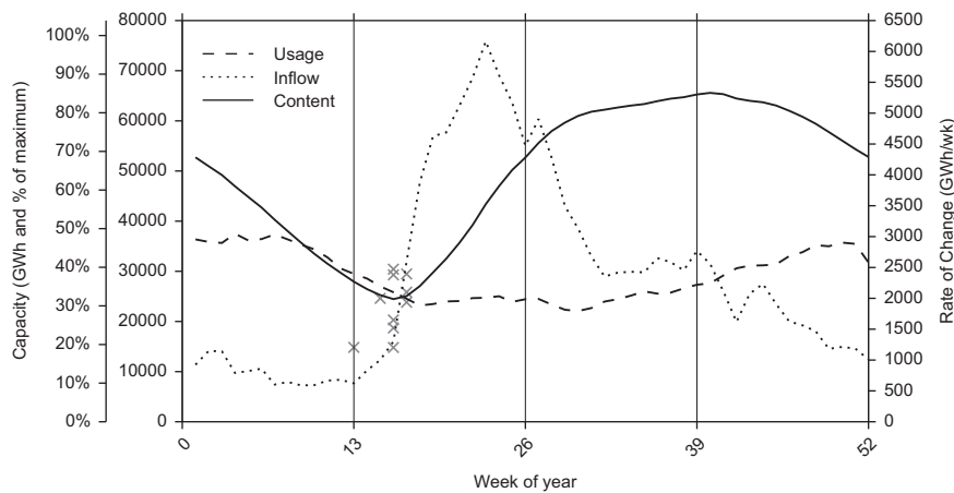
Fig. 4. The annual cycle of Norwegian hydropower, constructed from weekly inflow and content data for the period 2002–2010. Reservoir content valid for the end of the corresponding week is plotted according to the left hand axis, whilst inflow and usage totals valid for the corresponding week are plotted according to right hand axis. The usage in week i is derived using the expression usage_i = inflow_i - content_i + content_{i-1} . Grey crosses indicate the reservoir minima between 2002 and 2011.
