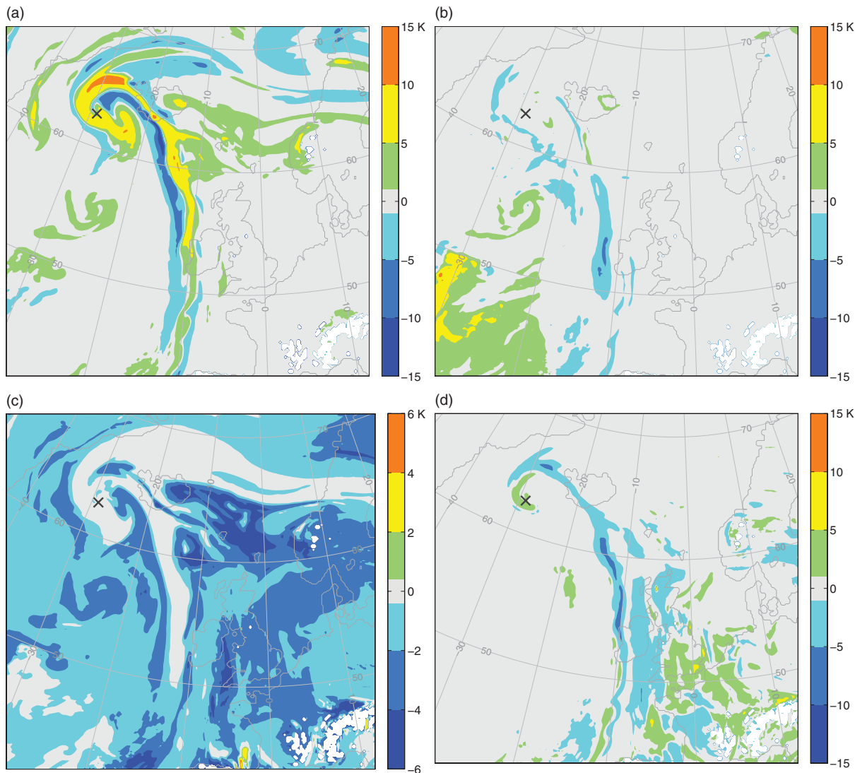
Figure 6. Parametrized diabatic process \theta -decomposition at \theta = 295 K at 0600 UTC on 30 September 2011: (a) \Delta\theta_{LS lb} , (b) \Delta\theta_{conv} , (c) \Delta\theta_{rad} (notice the different colour scale) and (d) \Delta\theta_{BLmix} . Black crosses indicate the position of the mean-sea-level low pressure centre.
