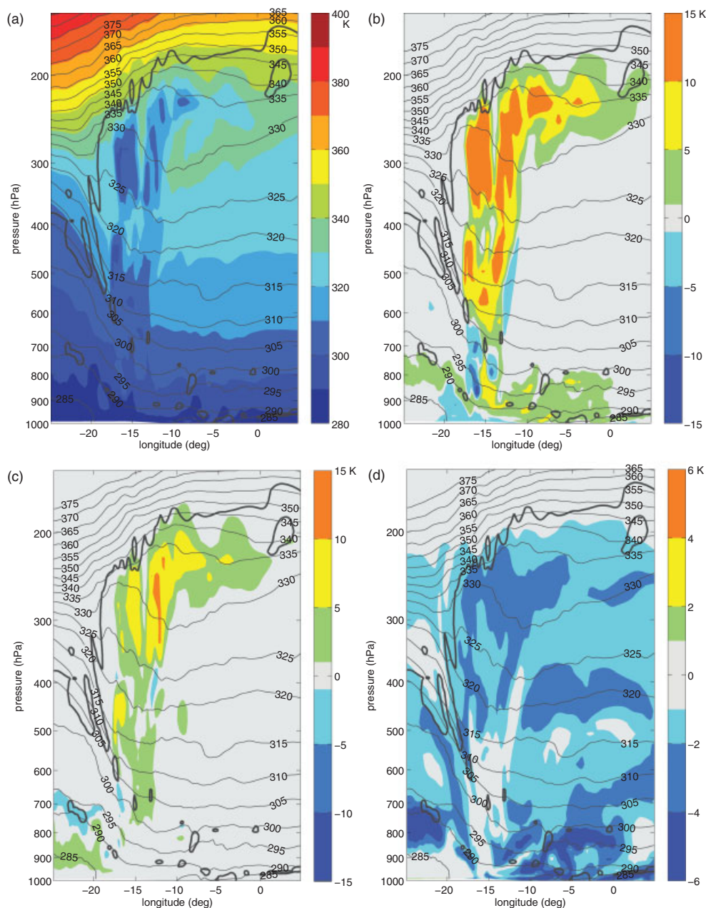
Figure 7. Vertical section along the segment AB indicated in Figure 3 for 0600 UTC on 30 September 2011 showing (a) \theta_0 , (b) \Delta\theta_{LSh} , (c) \Delta\theta_{conv} and (d) \Delta\theta_{rad} . Note the different colour scales used. Bold black lines represent the 2 PVU contour. Thin black lines represent potential temperature contours with a 5 K separation.
