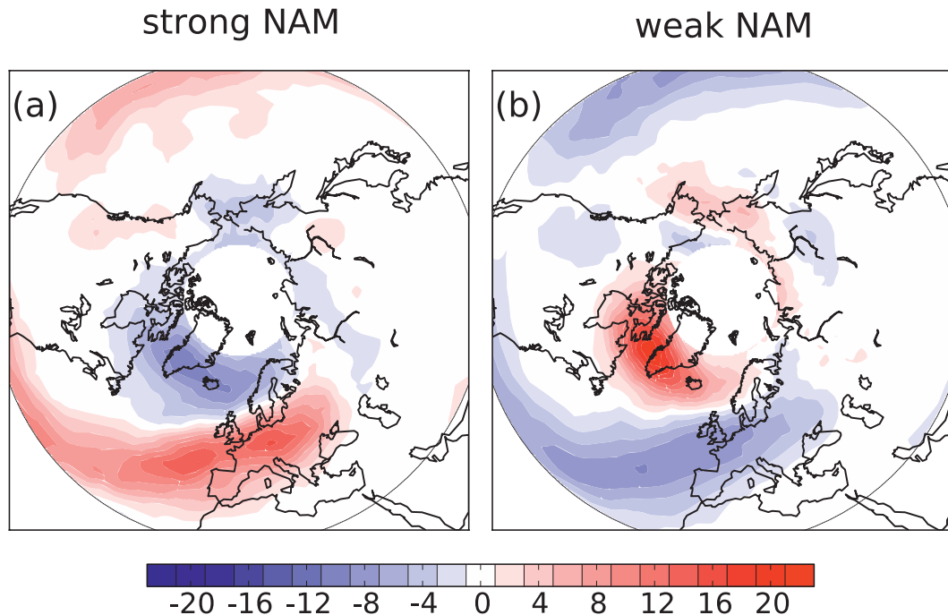
FIG. 10. Composites of deseasonalized blocking frequency at Z_{500} in the NH for (left) strong positive AO events and (right) strong negative AO events. Units are blocking frequency per day.
