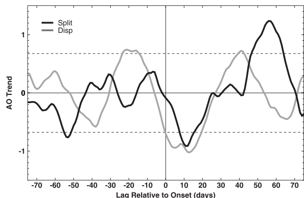
FIG. 6. Trend in the time series of the average AO for splits (black) and displacements (gray) \pm 15 days on either side of the lag day. Days are lagged relative to the event onset (day 0). Units are change in AO per month. Dashed lines show values of the AO trend which are significant at the 95% level using a Monte Carlo resampling test.
