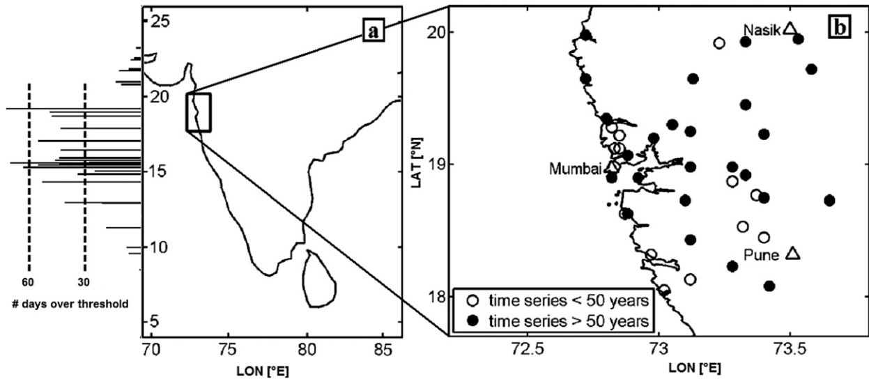
FIG. 1. (a) Study region (black rectangle) and number of days exceeding 15-mm daily precipitation accumulation during the 1951–87 period (histogram). (b) Location of precipitation gauges in the Mumbai area; the symbols distinguish the length of the available time series.
