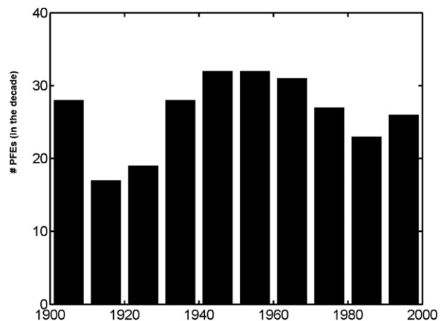
FIG. 5. Number of PFEs in each decade from 1900 to 2000.
