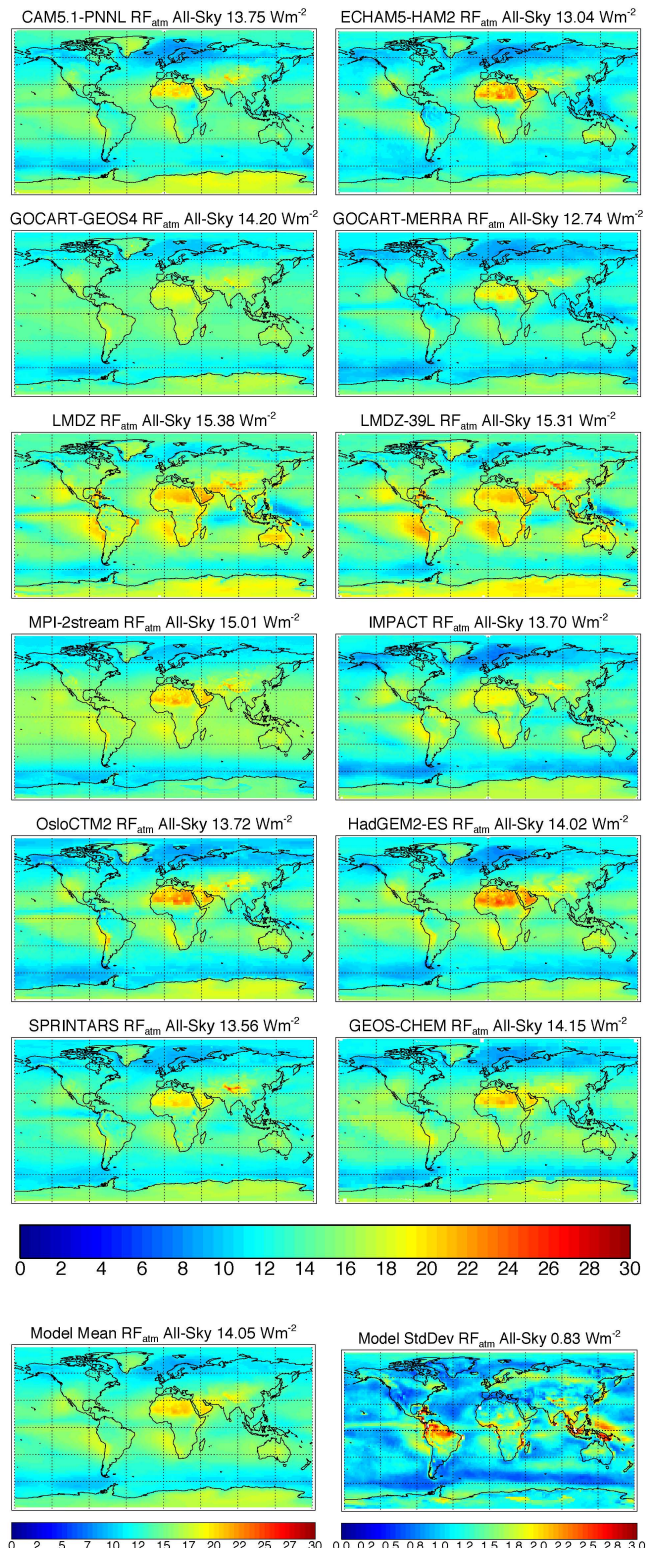
Fig. 15. Annual mean short-wave all-sky atmospheric radiative forcing (absorption) between experiments with SSA = 0.8 and SSA = 1.0 with holding ANG = 1.0 constant (FIX3-FIX2).
