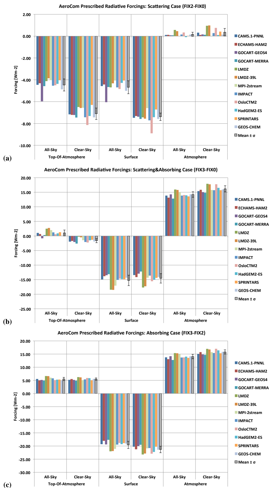
Fig. 16. Annual global-mean short-wave clear-sky and all-sky top-of-atmosphere, surface and atmospheric radiative forcing (absorption) between (a) experiments with AOD = 0.2 and AOD = 0.0 for SSA = 1.0, (b) experiments with AOD = 0.2 and AOD = 0.0 for SSA = 0.8 and (c) experiments with AOD = 0.2 for SSA = 0.8 and SSA = 1.0.
