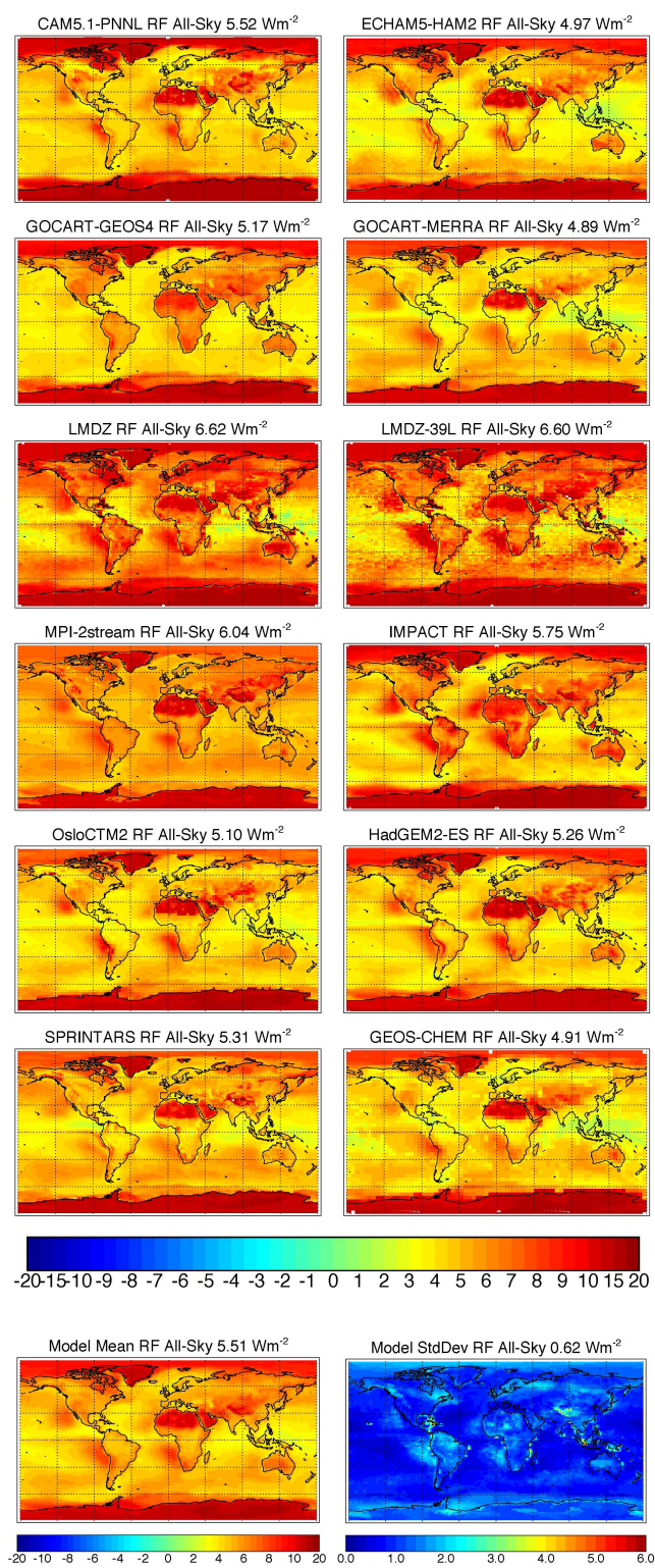
Fig. 13. Annual mean short-wave all-sky top-of-atmosphere radiative forcing (RF) with AOD=0.2 distributed over the lowest two kilometers between experiments with SSA = 0.8 and SSA = 1.0 with holding ANG = 1.0 constant (FIX3-FIX2).
