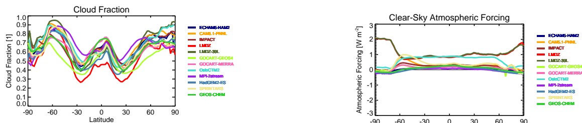
Fig. A1. Annual zonal-mean cloud fractions for experiment FIX0 (AOD = 0.0).
