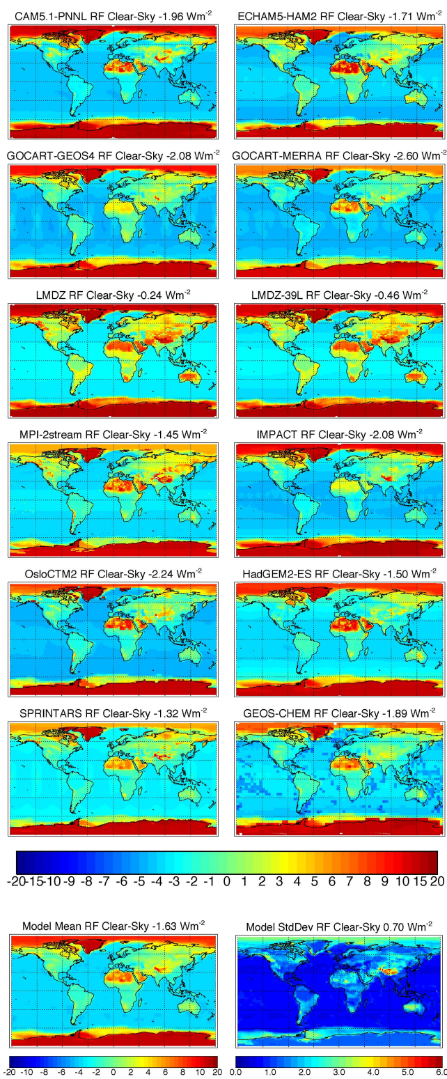
Fig. 8. Annual mean short-wave clear-sky top-of-atmosphere radiative forcing between experiments with AOD=0.2 and AOD=0.0 distributed over the lowest two kilometers, holding SSA = 0.8 and ANG = 1.0 constant (FIX3-FIX0).
