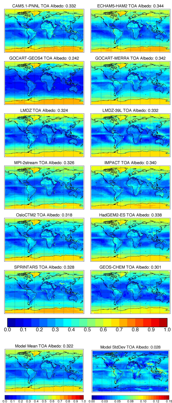
Fig. 4. Annual mean broadband short-wave top-of-atmosphere albedo for experiment FIX0 (AOD = 0.0).
