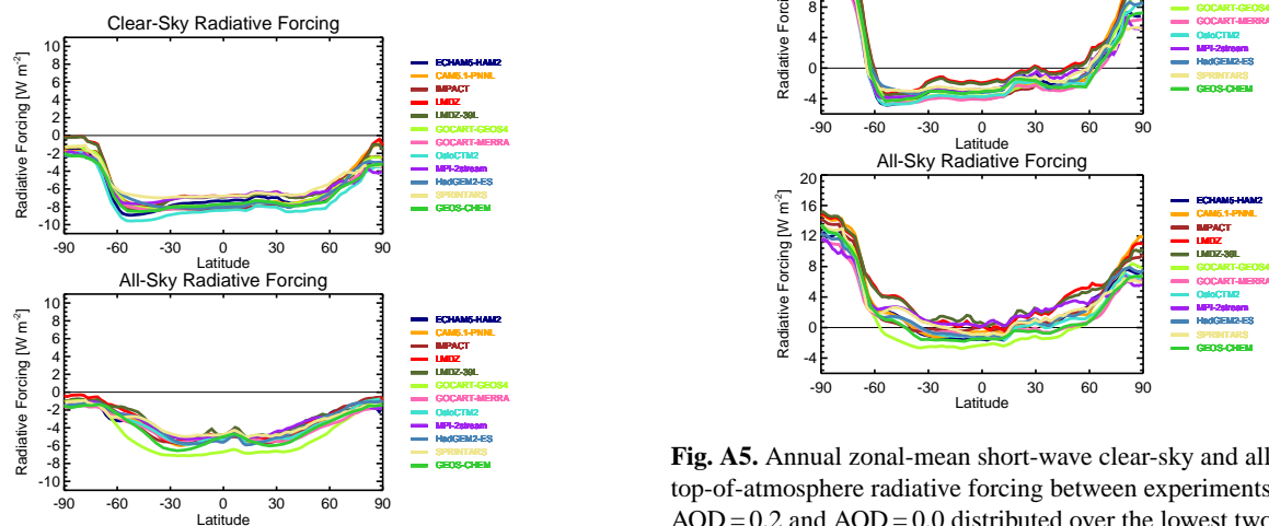
Fig. A3. Annual zonal-mean short-wave clear-sky and all-sky top-of-atmosphere radiative forcing between experiments with AOD = 0.2 and AOD = 0.0 distributed over the lowest two kilometers, holding SSA = 1.0 and ANG = 1.0 constant.
