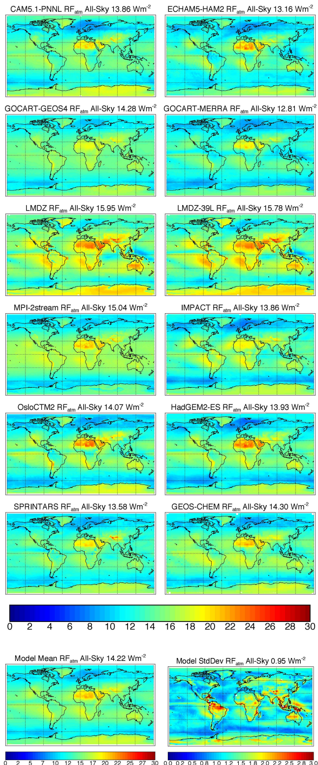
Fig. 11. Annual mean short-wave all-sky atmospheric radiative forcing (absorption) between experiments with AOD=0.2 and AOD=0.0 distributed over the lowest two kilometers, holding SSA = 0.8 and ANG = 1.0 constant (FIX3-FIX0).
