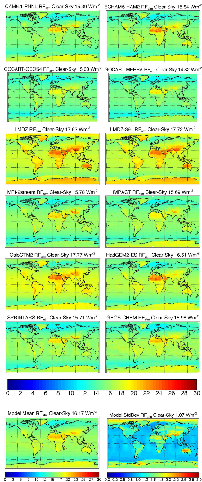
Fig. 10. Annual mean short-wave clear-sky atmospheric radiative forcing (absorption) between experiments with AOD=0.2 and AOD=0.0 distributed over the lowest two kilometers, holding SSA = 0.8 and ANG = 1.0 constant (FIX3-FIX0).
