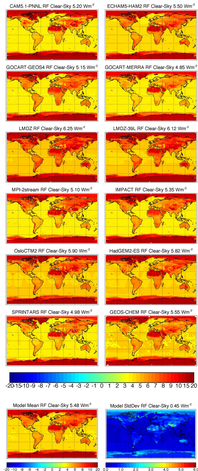
Fig. 12. Annual mean short-wave clear-sky top-of-atmosphere radiative forcing (RF) with AOD=0.2 distributed over the lowest two kilometers between experiments with SSA = 0.8 and SSA = 1.0 with holding ANG = 1.0 constant (FIX3-FIX2).
