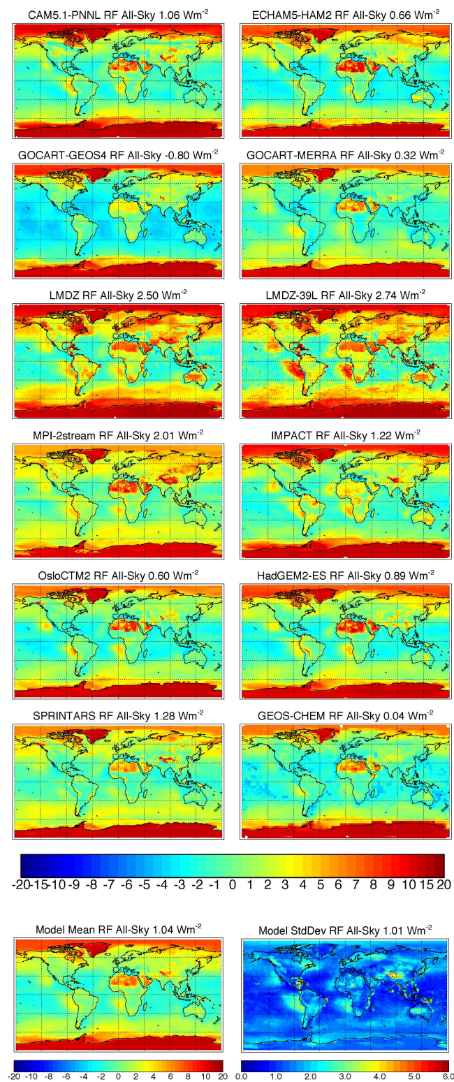
Fig. 9. Annual mean short-wave all-sky top-of-atmosphere radiative forcing between experiments with AOD=0.2 and AOD=0.0 distributed over the lowest two kilometers, holding SSA = 0.8 and ANG = 1.0 constant (FIX3-FIX0).
