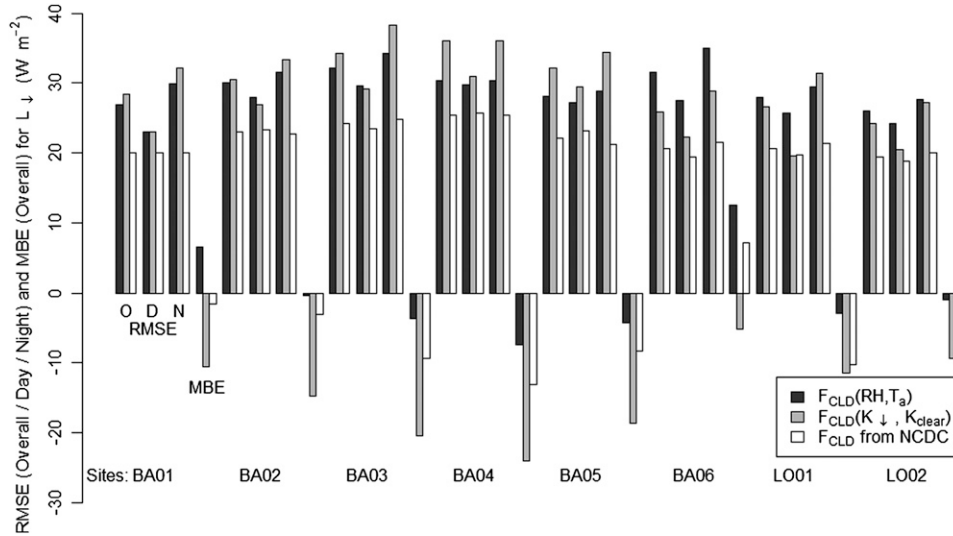
FIG. 3. The RMSE (analyzed for all-daytime–nighttime hours) and MBE (all hours only) when modeling L_{\downarrow} for Baltimore (2002–06, BA01–BA06) and Łódź (2001–02, LO01 and LO02) using options (a), (b), and (c) given in Fig. 2.
