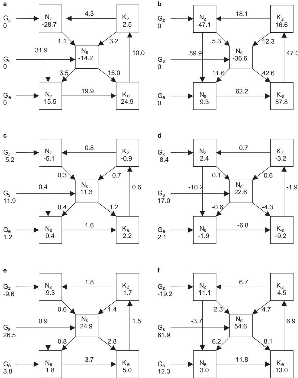
Fig. 6a–f. Energy box diagnostics showing rates of change and conversions between different forms of energy (units 10^3 \text{J m}^{-2} \text{day}^{-1} ) for three life cycle experiments: a, b DRY; c, d the anomaly G100ST60-DRY and e, f the anomaly G100-DRY. Values given are averages over days 5 to 7 ( a, c, e ) and days 8 to 10 ( b, d, f )
