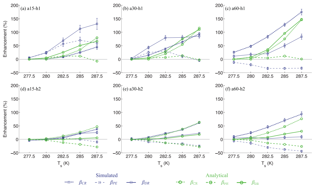
Figure 10. Simulated (black, blue online) and analytically derived (grey, green online) \beta for each of the non-dimensional diagnostics (Eq. (34)). The cases (a) a15-h1, (b) a30-h1, (c) a60-h1, (d) a15-h2, (e) a30-h2 and (f) a60-h2 are shown. In each panel, \beta_{\mathbb{C}\mathbb{R}} and \beta_{\mathbb{C}\mathbb{R}_i} are dotted, \beta_{\mathbb{P}\mathbb{E}} and \beta_{\mathbb{P}\mathbb{E}_i} are dashed and \beta_{\mathbb{D}\mathbb{R}} and \beta_{\mathbb{D}\mathbb{R}_i} are solid. Error bars are as in Figure 5. This figure is available in colour online at wileyonlinelibrary.com/journal/qj
