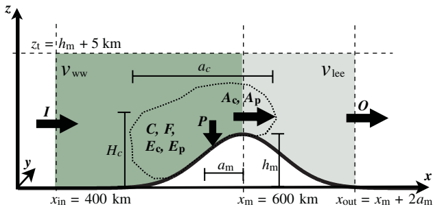
Figure 2. A schematic showing the fluxes and conversion rates of water substance in the simulations of Cannon et al. (2012). Symbols are as defined in the text. This figure is available in colour online at wileyonlinelibrary.com/journal/qj
