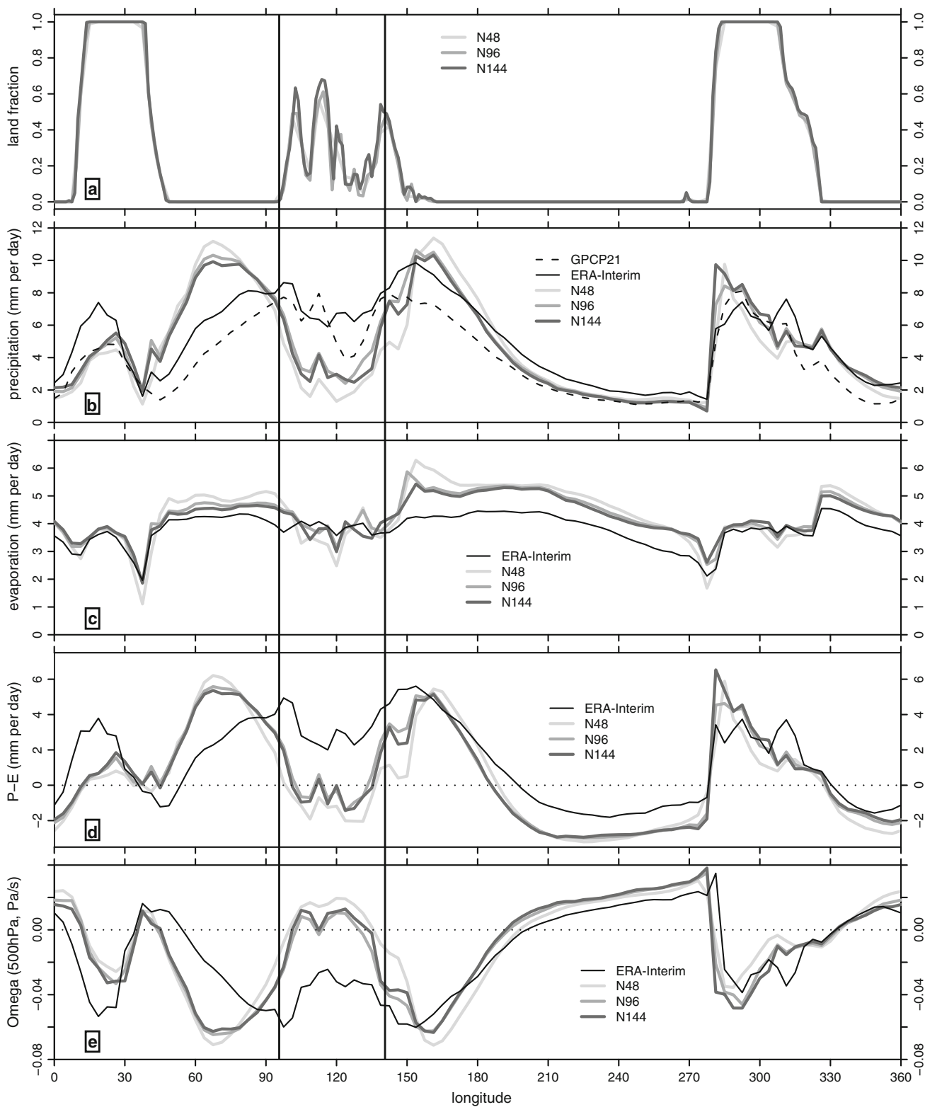
Fig. 3 Mean values of a land fraction, b precipitation P , c evaporation E , d P-E , and e midtropospheric vertical velocity in a tropical channel ( -8.75 to 3.75^\circ\text{N} ) versus longitude. Vertical lines shown the analysis domain ( 95.625 – 140.625^\circ\text{E} )
