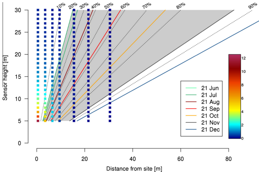
Fig. 5. Schematic of source area variations for a down-facing pyranometer depending on sensor height above roof and distance from site. Points give source area contribution of flat 1 \text{ m}^2 roof window [%] according to concentric footprint isopleths (Schmid et al., 1991), indicated by dotted lines. Solid lines mark location of minimum radius of specular reflection R_s on the 21st of each month (Jun–Dec), calculated for a site at 50^\circ \text{ N} . See Section 3.2.
