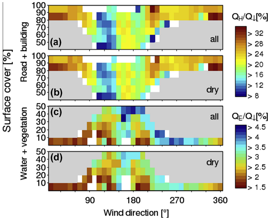
Fig. 8. Median heat flux (a, b) Q_H and (c, d) Q_E at KSS normalised by incoming radiation Q_i by wind direction and surface cover; (a, c) all conditions; (b, d) restricted to periods with no rain within the preceding 12 h. Minimum number of measurements available to calculate the median for each interval (a, b) 15; (c, d) 20 (white – insufficient data). Grey shading indicates land cover/wind direction combinations that cannot occur.
