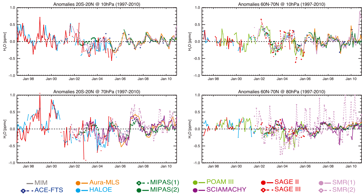
Figure 10. Time series of deseasonalized water vapor anomalies at (left) 10 and 70 hPa in the tropics ( 20^{\circ}\text{S} – 20^{\circ}\text{N} ) and at (right) 10 and 80 hPa in the extratropics ( 60^{\circ}\text{N} – 70^{\circ}\text{N} ) between 1997 and 2010.
