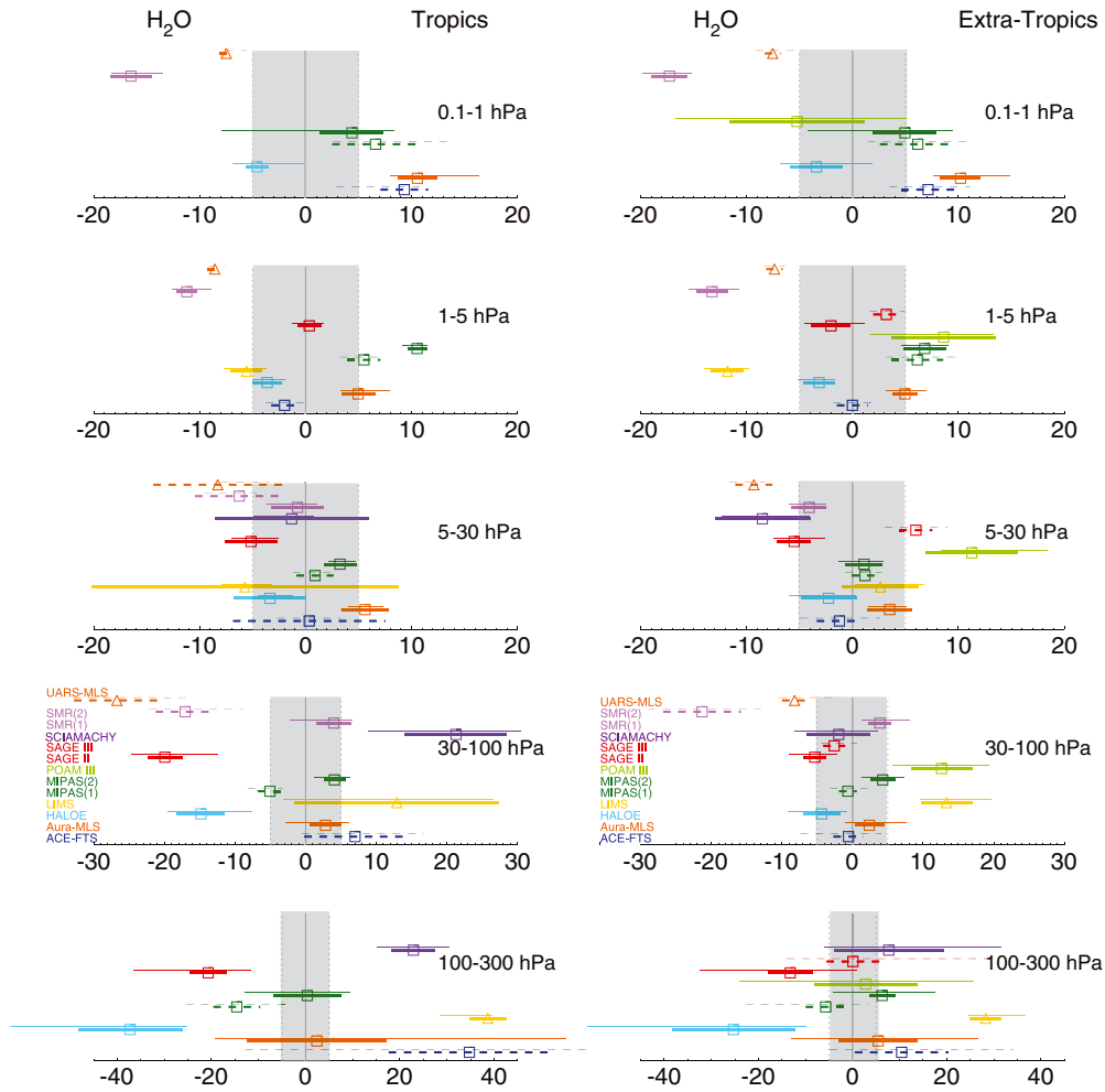
Figure 16. Interinstrument differences in water vapor calculated for the tropics (left) ( 20^{\circ}\text{S} – 20^{\circ}\text{N} ) and (right) extratropics ( 40^{\circ}\text{S} – 80^{\circ}\text{S} and 40^{\circ}\text{N} – 80^{\circ}\text{N} ) and for five different altitude regions from the UT up to the LM. Shown are the median (squares), median absolute deviations (MAD, thick lines), and the mean \pm 1\sigma ranges (thin lines) of the relative differences between each individual instrument and the MIM calculated over a given latitude and altitude region. The reference period is 1998–2008 and based on the results of section 4.1.3. Triangles indicate medians of instruments that are obtained outside of the reference period: LIMS and UARS-MLS are shown with respect to the instrument means of SAGE II and HALOE based on comparisons for 1978–1990 and 1991–1993, respectively.
