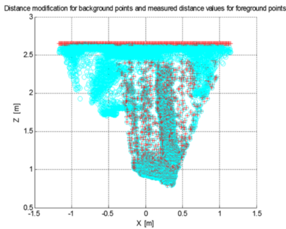
Figure 12 Foreground and background Z values from ToF points in ToF camera frame. Background distance modification of distance values. View of axis x, z .
