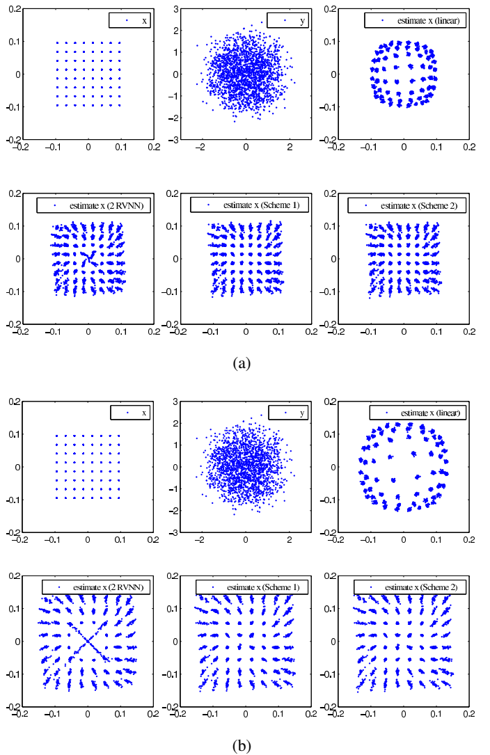
Fig. 5. Effectiveness of the proposed nonlinear SC-FDE scheme based on the estimated CIR \hat{h} and the estimated HPA's CV static nonlinearity as well as the estimated inverse mapping for the HPA's CV nonlinearity under: (a) OBO = 3 dB, E_b/N_o = 4 dB; and (b) OBO = 2 dB, E_b/N_o = 10 dB. The top three plots in the two sub-figures (a) and (b) depict one transmitted QAM symbol block x , its received signal block y , and the corresponding estimated \hat{x} obtained by the linear SC-FDE. The bottom three plots in (a) and (b) show the estimated \hat{x} obtained by the previous 2RVNN based SC-FDE [38] and the current CVNN based SC-FDE using the two proposed schemes, respectively.
