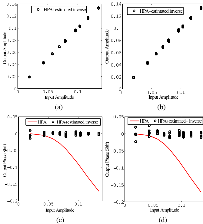
Fig. 4. Combined response of the true HPA and its estimated inversion obtained under OBO = 3 dB and E_b/N_o = 4 dB: (a) combined amplitude response by Scheme 1; (b) combined amplitude response by Scheme 2; (c) combined phase response by Scheme 1; and (d) combined phase response by Scheme 2.
