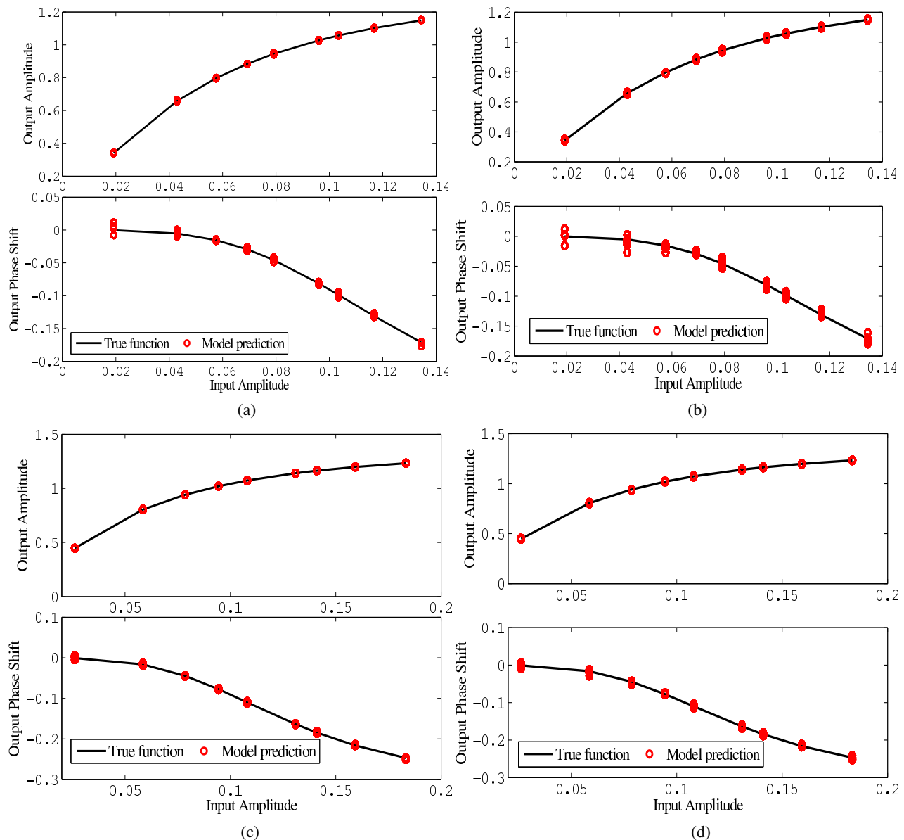
Fig. 3. Comparison of the HPA's nonlinearity \Psi(\cdot) and the estimated nonlinearity \hat{\Psi}(\cdot) : (a) Scheme 1 under OBO=3 dB, E_b/N_o = 4 dB; (b) Scheme 2 under OBO=3 dB, E_b/N_o = 4 dB; (c) Scheme 1 under OBO=2 dB, E_b/N_o = 10 dB; and (d) Scheme 2 under OBO=2 dB, E_b/N_o = 10 dB.
