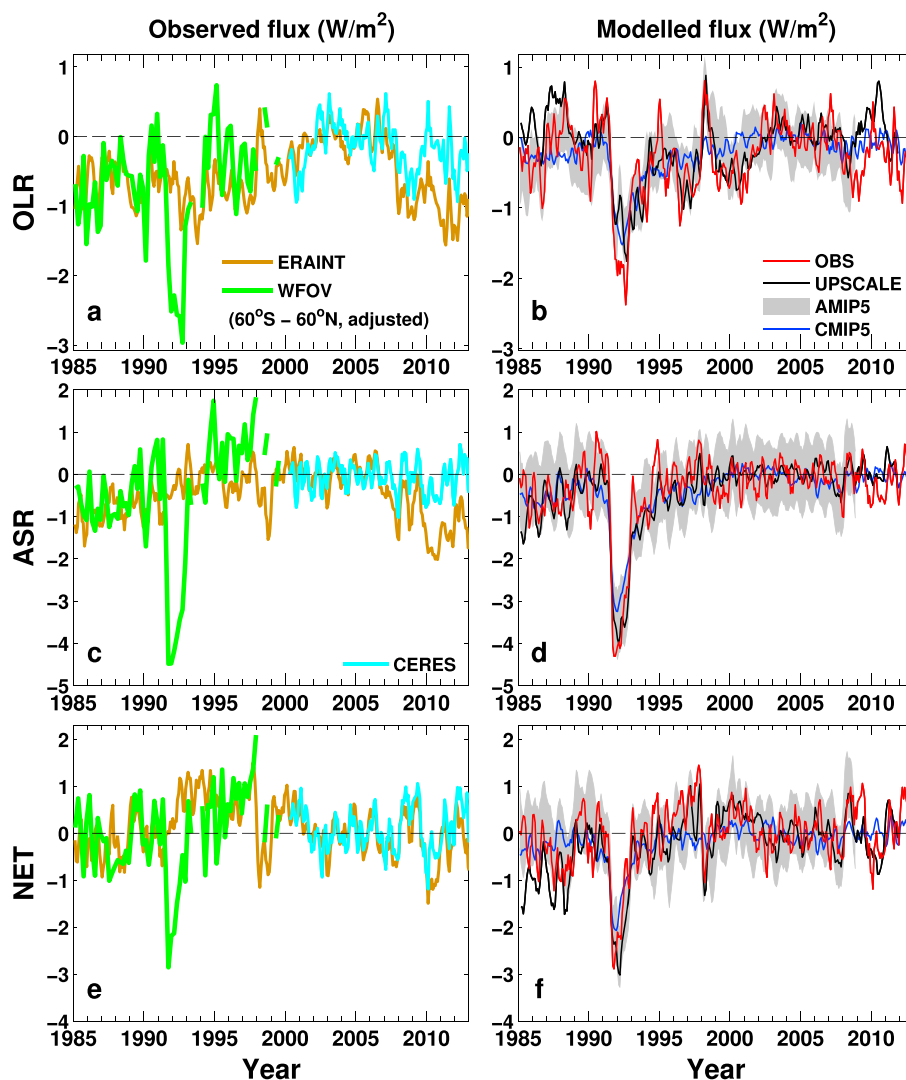
Figure 2. Changes in (a, c, e) observed and (b, d, f) simulated/reconstructed global mean deseasonalized anomalies (relative to the 2001–2005 period) of outgoing longwave radiation (Figures 2a and 2b), absorbed solar radiation (Figures 2c and 2d), and net downward radiation at the top of the atmosphere (Figures 2e and 2f). Three-month running means are applied. Gray shading denotes the \pm 1 standard deviation of the nine AMIP5 simulations. WFOV 72 day mean data are deseasonalized with respect to the 1985–99 period and for clarity is adjusted so multiannual 60°S–60°N mean anomalies match corresponding ERAI global mean anomalies (Figures 2a, 2c, and 2e).
