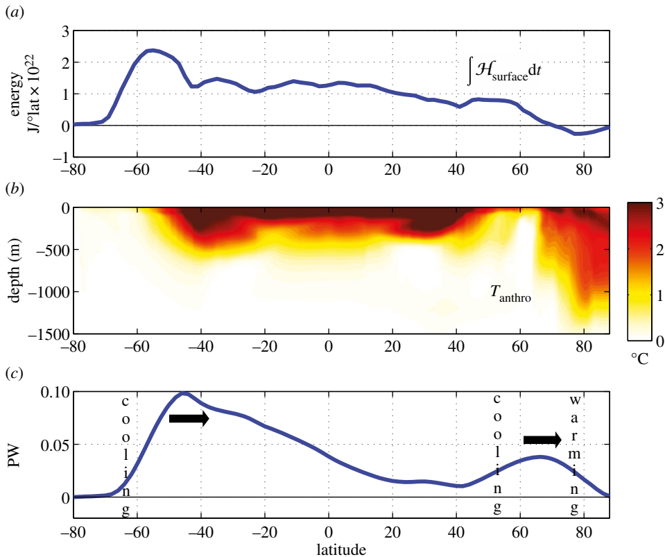
Figure 4. (a) Surface energy accumulation integrated over 100 years in \text{J}/^\circ\text{lat} \times 10^{22} . (b) Meridional section of zonal-average T_{\text{anthro}} after 100 years from the ocean-only configuration of MITgcm whose \text{SST}_{\text{anthro}} is shown in figure 2b. (c) Anomaly in meridional ocean heat transport (in PW) after 100 years relative to a control integration. Latitudinal bands of implied ocean warming and cooling are marked.
