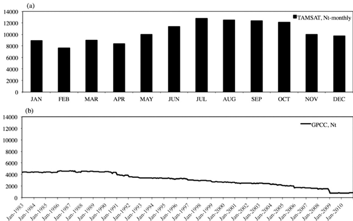
FIG. 3. Total number of gauges N_t (a) used in the TAMSAT climatology-based calibration (varying monthly but not interannually) and (b) in the GPCCC archive (varying over time and exhibiting a nearly fourfold reduction from 1983 to 2010).
