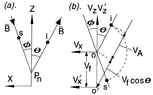
Figure 3. (a) The rotational discontinuity (RD) formed by a newly opened field line at P_n which evolves along the magnetopause in the Z direction at speed V_f in the Earth's frame of reference. The X direction is the outward normal to the boundary. (b) A velocity space plot showing field-aligned bulk flow at the Alfvén speed, V_A , in the de Hoffmann-Teller frame ( V_x, V_z with origin at O) both into the RD in the magnetosheath (at s) and away from the RD in the magnetosphere (at i). This geometric construction allows the calculation of the minimum and bulk flow field-aligned speed of injected particles in the Earth's frame ( V_x', V_z' with origin at O'). (Adapted from Cowley [1982]).
