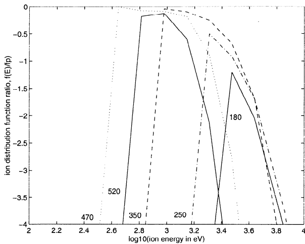
Figure 10. Averages of ideal spectra (of the kind shown in Figure 9) over 0.7-s ranges of elapsed time ( t_s - t_o ) and energy channels \delta E = 0.1 E wide, where the center energies, E are given in the text. Comparison with Figure 9 reveals the effects of time and energy averaging and coarse energy resolution.
