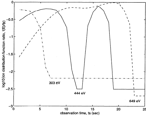
Figure 12. Modeled variations of f(t_s) from the spectra shown in Figure 11, for three of the logarithmically spaced energy channels centered on the energies ( E ) given. In all cases, the decay of f from its peak value is shown as the satellite emerges through the equatorward edge of the cusp/cleft precipitation when E = E_{ic} .
