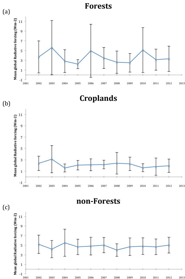
Figure 4. The mean annual radiative forcing per land cover (a–c) in Wm^{-2} .
