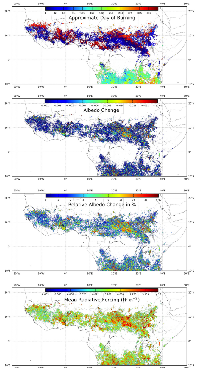
Figure 5. The approximate day of burning; the “instantaneous” shortwave albedo change in areas affected by fire; the relative change in albedo in %; and the associated radiative forcing in Wm^{-2} is shown for the Sahel during 2003.
