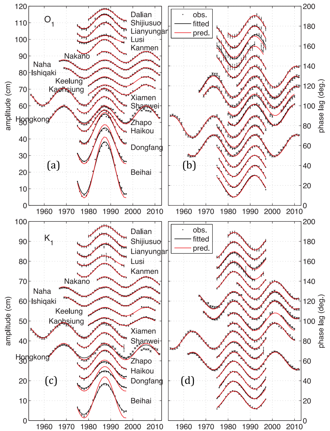
Figure 5. (left) Time series of tidal amplitude and (right) phase lag for major lunar constituents (a and b) O_1 and (c and d) K_1 . Black dots present annual values with error bars at 95% confidence level obtained from the harmonic analysis of each 1 year of hourly data. Black and red solid lines are the best fitted curve and theoretical nodal modulation, respectively. Note that the series have been offset for display. Parameters of the best estimations (black solid lines) are presented in the supporting information Tables S1 and S2.
