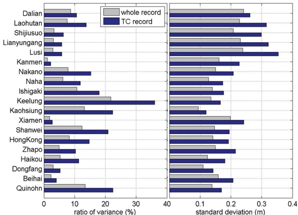
Figure 2. The ratio of variance of tidal residual over (a) the variance of sea level and (b) the standard deviation of tidal residual, for the whole record (gray) and for only the TC-influenced record (blue).
