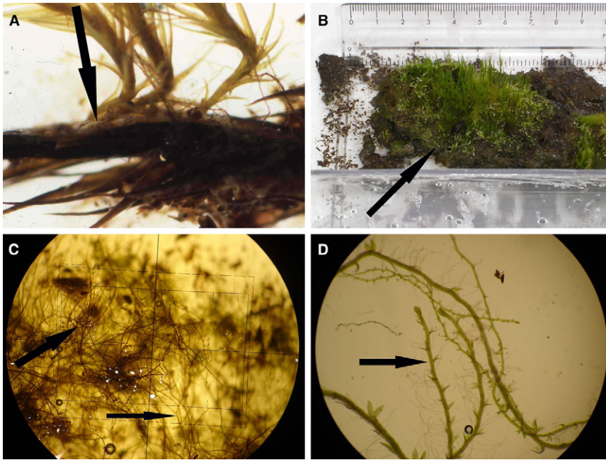
Figure 1. Moss regrowth at different depths in the core. (A) Site of new growth emerging from existing gametophytes on the fresh-cut face of the core at 110 cm depth (arrow). (B) Extensive regrowth of Chorisdontium aciphyllum from the basal section of the core at 121–138 cm depth. (C) Regrowth from the basal section of the core, showing preserved brown rhizoids (thick arrow) and new protonemal growth (thin arrow). (D) New shoots of the liverwort Cephaloziella sp.
