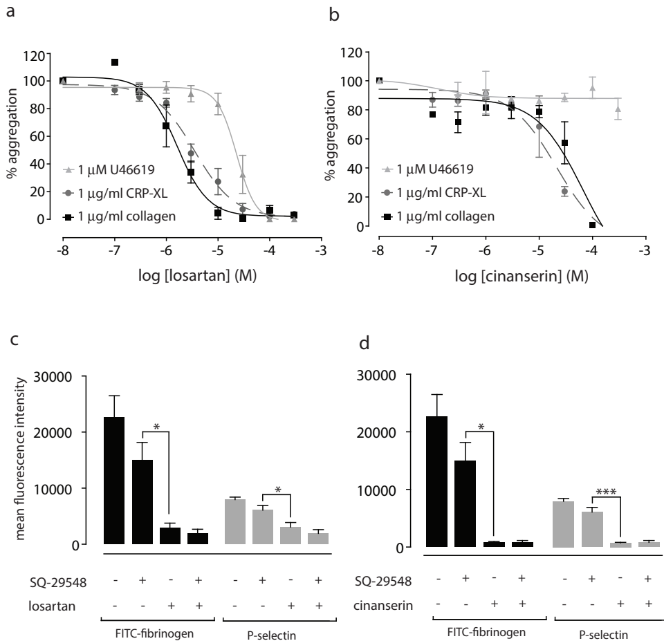
Figure 4. Losartan is selective for GPVI over TPR. To assess effects on TPR signalling, platelets were activated with 1 \mu\text{M} U46619 and aggregations followed for 5 minutes in the presence of or absence of drug ( n=3 , \pm SEM). Collagen (solid black line) and CRP-XL (dashed dark grey line) were both used at 1 \mu\text{g}/\text{ml} . Losartan (a) has an \text{IC}_{50} of \sim 20 \mu\text{M} for U46619-induced aggregation (solid grey line) while cinanserin (b) has no effect on TPR signalling (solid grey bar). Exposure of P-selectin (CD62P) and FITC-fibrinogen binding was measured by flow cytometry. Losartan (100 \mu\text{M} , c) and cinanserin (100 \mu\text{M} , d) both reduce FITC-fibrinogen binding (black bars) and P-selectin exposure (grey bars) compared to SQ-29548 alone. Statistical analysis was conducted by one-way ANOVA with Sidak's multiple comparisons correction. ns P>0.05 , * P<0.05 , *** P<0.001 , n=3 , \pm SEM.
