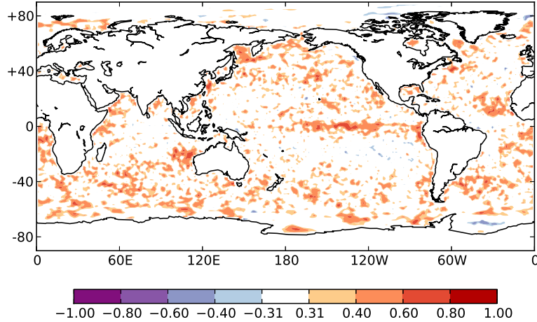
(b) Initial SST discrepancy, 12h 1000hPa temperature shock correlation, M1
