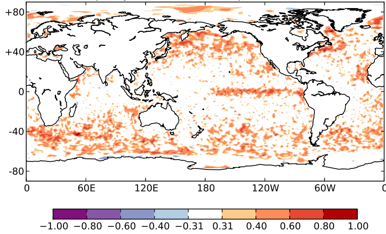
(a) Initial SST discrepancy, 12h 1000hPa temperature shock correlation, U1
