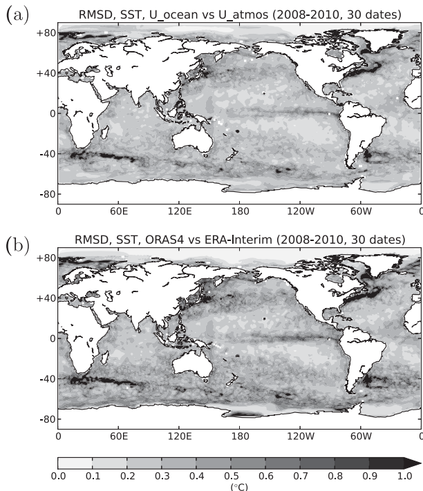
FIG. 2. (a) Root-mean-square difference between U_{\text{ocean}} SST and the SST used as forcing by U_{\text{atmos}} , at the beginning of the forecasts, showing the imbalance present in the initialization of forecasts U1. (b) As in (a), but for ORAS4 and ERA-Interim, showing one of the sources of imbalance in the initialization of forecasts M1.
