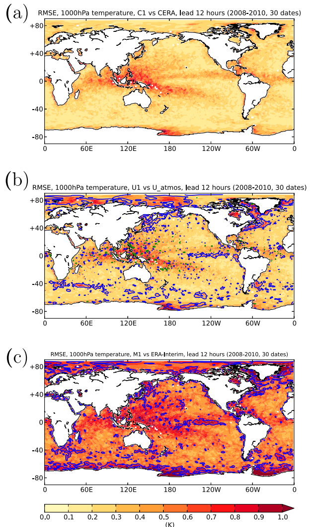
FIG. 3. 1000-hPa temperature forecast RMSE, relative to the analysis used as the initial conditions, for (a) C1, (b) U1, and (c) M1, at 12-h lead time. Land areas are masked out, as the focus is on atmosphere–ocean imbalance. Contours in (b) and (c) show differences in RMSE relative to C1, with blue (green) contours marking increased (decreased) RMSE in U1 and M1. Contours are drawn at differences of 0.15^{\circ}\text{C} in (b), and at differences of 0.5^{\circ}\text{C} in (c). Only differences that are significant at the 90% level, estimated using the bootstrapping method, are contoured.
