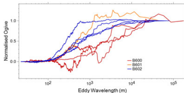
Figure 10. Ogives from flux measurements of the B600, B601, and B602 Harmattan wind cases. Each ogive represents one flux measurement, and the steeper regions of the curves indicate the scales which contribute to the flux. The ogives have been normalized to unity at the largest wavelength. Ogives are only plotted for flux measurements where the uncertainty is less than 100%, i.e., where there is a statistically significant flux.
