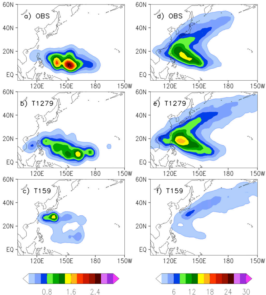
FIG. 2. (left) Genesis and (right) track densities of tropical cyclones equivalent to hurricanes of categories 1–5 as number density per season per unit area equivalent to a 5^{\circ} spherical cap for (a),(d) IBTrACS (OBS), (b),(e) AMIP T1279, and (c),(f) AMIP T159 based on MJJASON of 1975–2007.
