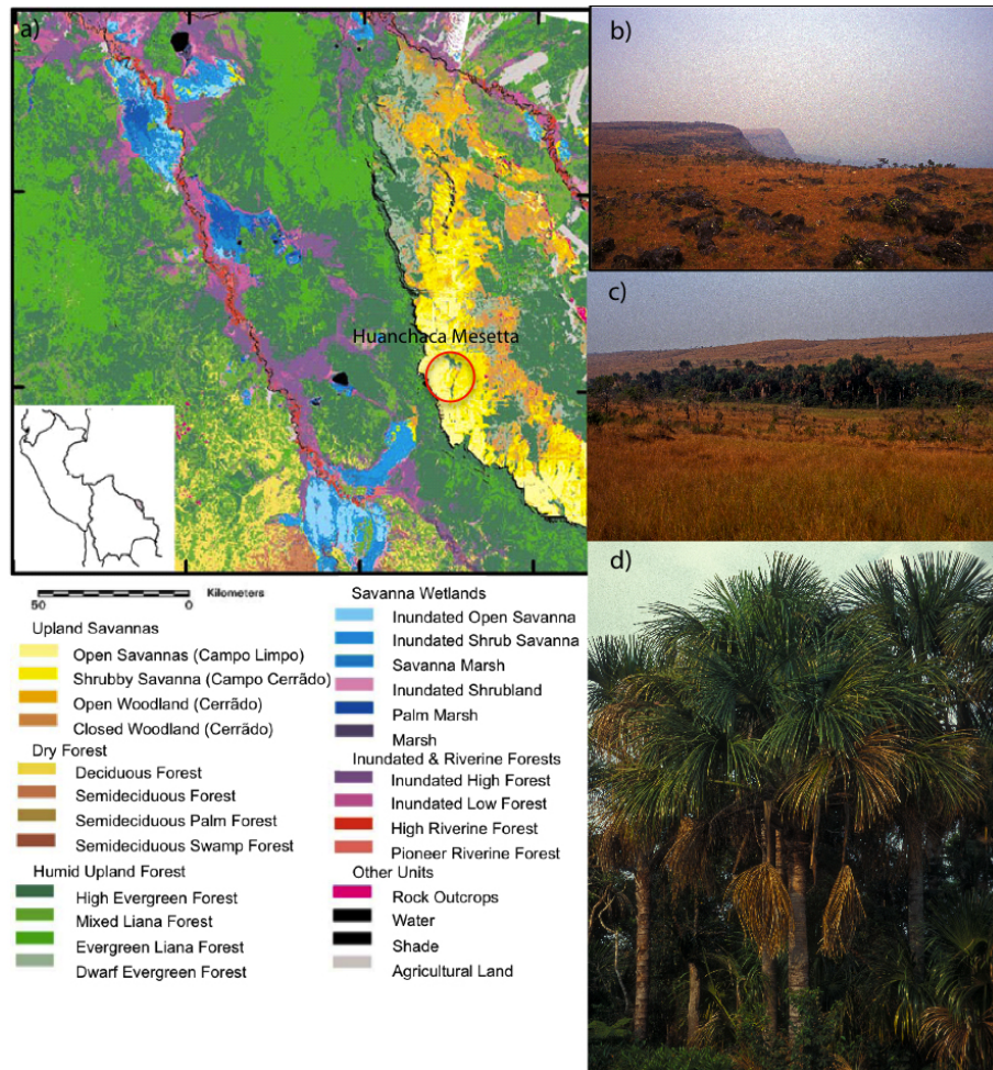
Figure 1. Huanchaca Mesetta study site (a) vegetation map of Noel Kempff Mercado National Park (NKMNP) modified from Killeen (1998b), (b) view from atop Huanchaca Mesetta, (c) Huanchaca Mesetta palm swamp, and (d) monospecific stand of Mauritia flexuosa . Photos by F. Mayle.
