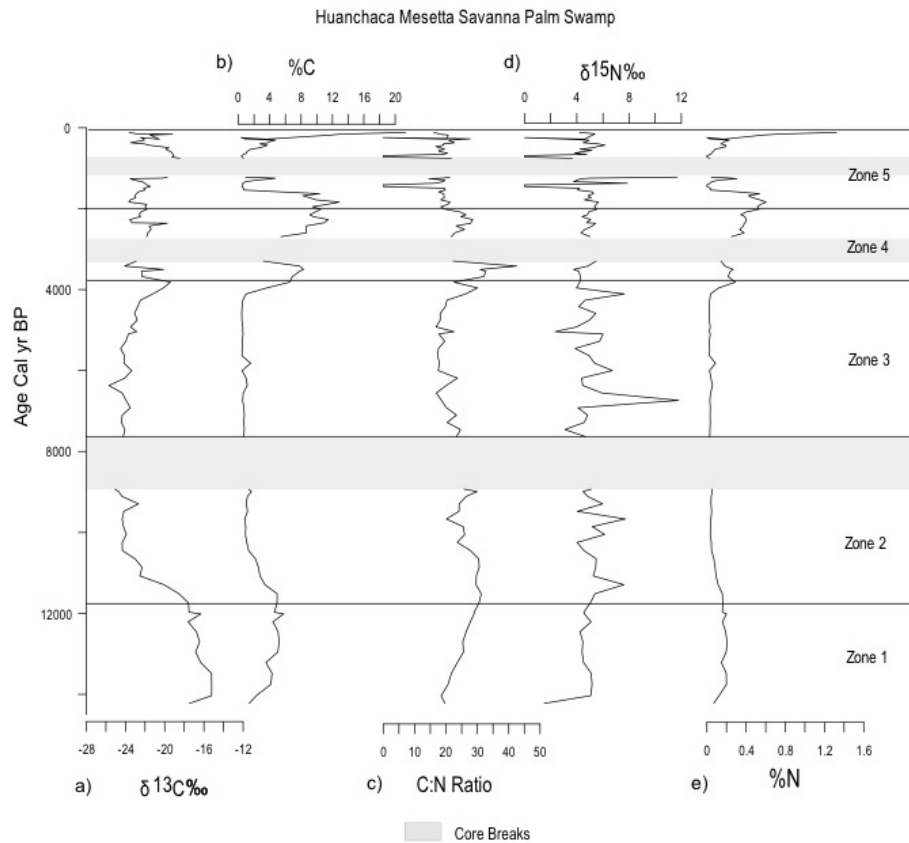
Figure 5. Huanchaca Mesetta stable isotope data: (a) \delta^{13}\text{C} , (b) % total carbon, (c) carbon to nitrogen ratio, (d) \delta^{15}\text{N} , and (e) % total N. Zones derived from phytolith data. Grey bars indicate core breaks.
