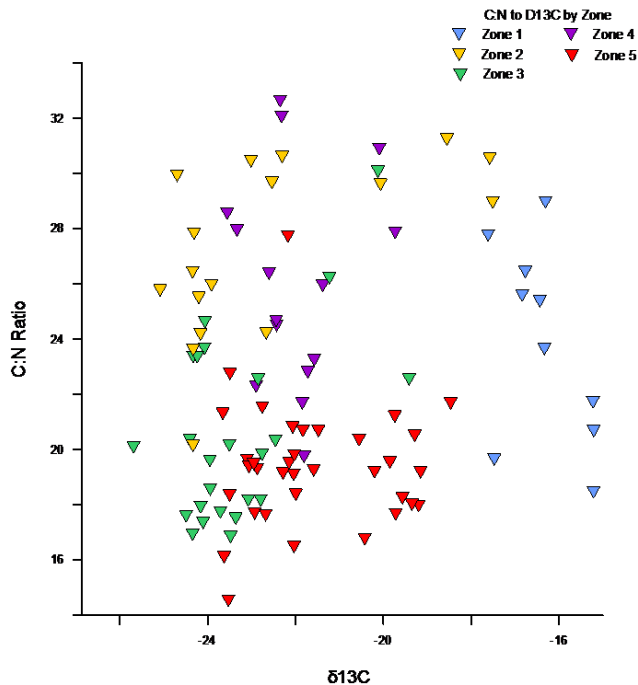
Figure 6. C:N ratio to \delta^{13}\text{C} stable isotopes by zones determined from phytolith data.
