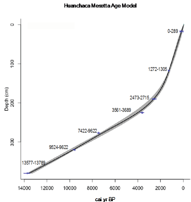
Figure 2. CLAM age–depth model for Huanchaca Mesetta. Grey bars represent 2σ error.
