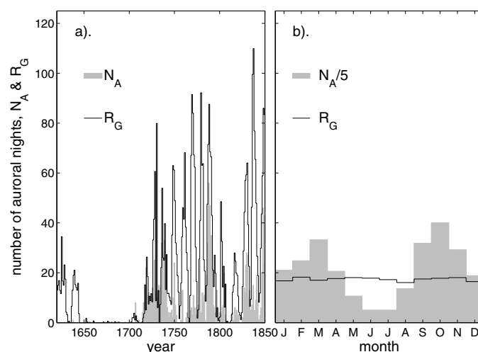
Fig. 10. Panel A) number of auroral nights, N_A , in calendar years for observations in Great Britain collated by E. J. Lowe (1870) with the addition of the observations by Thomas Hughes (Harrison 2005) and John Dalton (Dalton 1834) (grey histogram). Annual group sunspot number of Hoyt & Schatten (1998), with the adoption of recent corrections by Vaquero et al. (2011) and Vaquero & Trigo (2014) (black line). Lowes personal copy of his catalogue of natural phenomena (including auroras) was only recently discovered and was compiled completely independently of other catalogues. Yet it shows, like the others, the dearth of sightings during the MM, some events in 1707 and 1708 and the return of regular sightings in 1716. Panel B) annual variation of N_A in the same dataset and of R_G .
