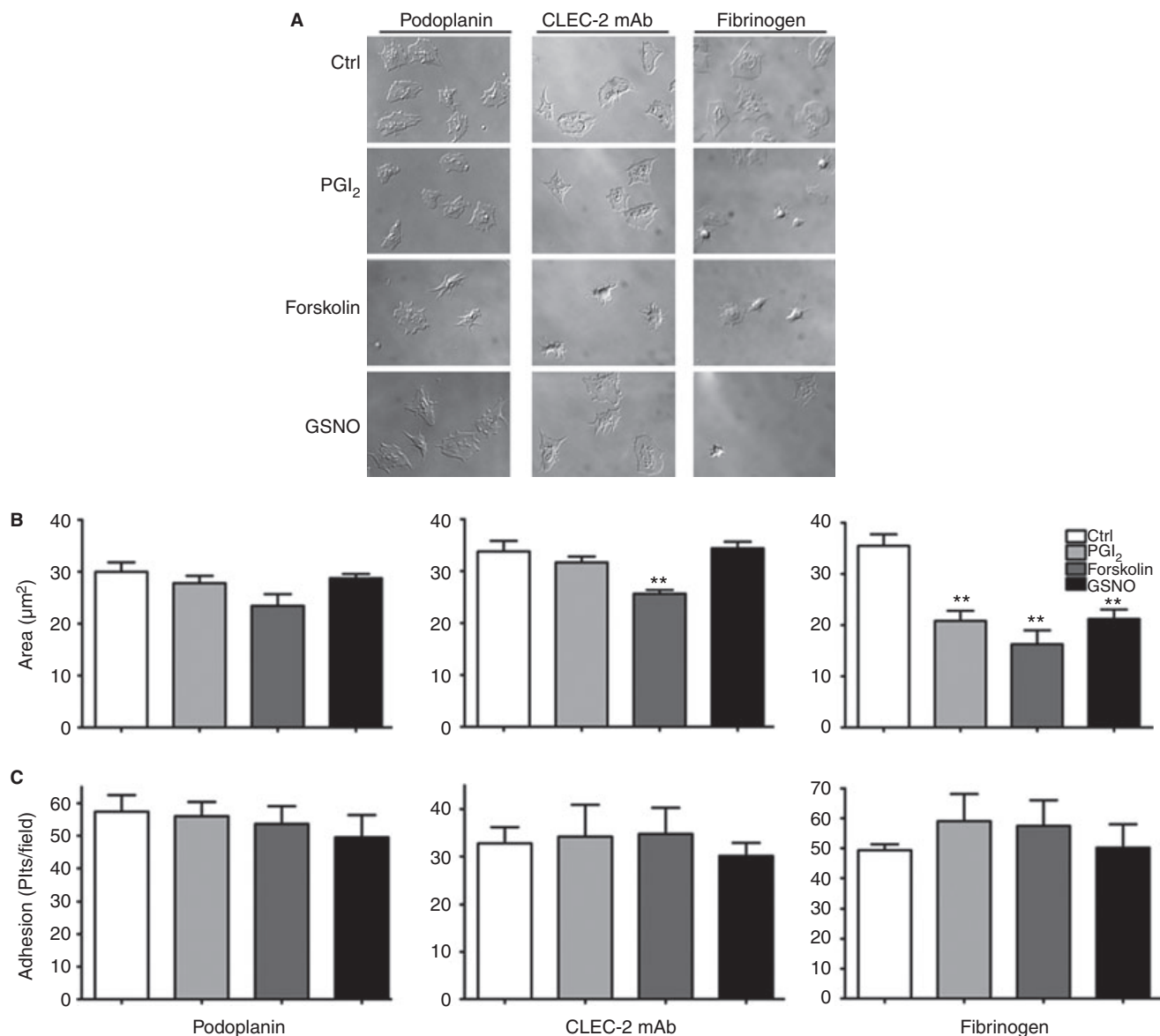
Fig. 4. cAMP-elevation marginally affects CLEC-2-dependent spreading. 2 \times 10^7 per mL washed platelets were treated with PGI 2 (1 µM), forskolin (10 µM) or GSNO (1 mM) before spreading on coverslips coated with 10 \mu\text{g mL}^{-1} recombinant podoplanin or CLEC-2 mAb. Control experiments with thrombin-activated platelets ( 0.1 \text{ U mL}^{-1} ) on 100 \mu\text{g mL}^{-1} fibrinogen were performed. Coverslips were imaged using differential interference contrast (DIC) microscopy (A). Platelet areas are expressed as mean of mean area/experiment \pm SEM. One hundred platelets/experiment were analyzed. Statistical differences were evaluated by ANOVA and Dunnet's post-test (** P < 0.01 ) (B). Results are expressed as mean of mean number of platelets/experiment \pm SEM ( n = 3-6 ) (C).
