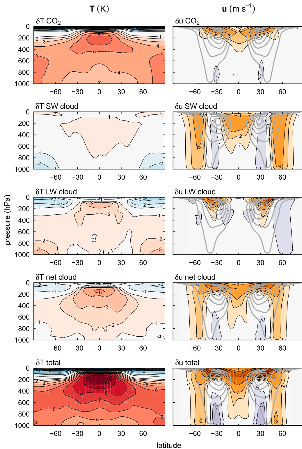
FIG. 3. (left) Temperature and (right) zonal wind responses to \text{CO}_2 quadrupling, broken down into contributions from \text{CO}_2 forcing and clouds. Shading denotes the response. In the right column, thick gray contours represent the control climatology (contour interval 10 \text{ m s}^{-1} , only positive values shown). The \text{CO}_2 , SW cloud, and LW cloud effects are calculated with Eqs. (2), (3), and (4), respectively.
