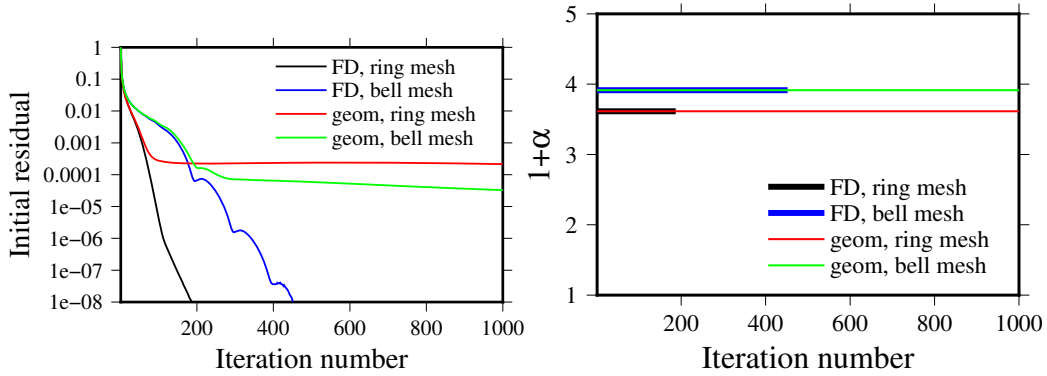
Figure 5: Convergence of initial residual of the solution of the Poisson equation for each fixed point iteration and 1 + \alpha as a function of iteration number for the planar meshes generated with the monitor function defined in eqn. (37).
