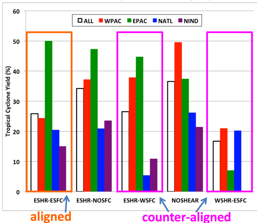
Figure 2. Histograms of the yield of tropical cyclones in each basin, defined as the number of tropical cyclones divided by the total number of tracked disturbances. White bars: total for each flow configuration; red for Western Pacific; green for Eastern Pacific; blue for Atlantic; and purple for Northern Indian Ocean. ESHR=easterly shear (850-200 hPa) greater than 2.5 \text{ m s}^{-1} ; WSHR=westerly shear; ESFC=easterly surface greater than 1.0 \text{ m s}^{-1} ; NOSFC=surface winds weaker than 1.0 \text{ m s}^{-1} ; NOSHEAR=shear less than 2.5 \text{ m s}^{-1} . Environmental flows are computed after removal of the vortex.
