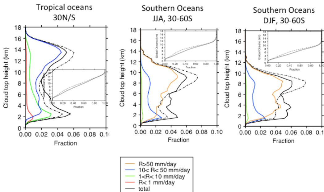
Figure 7. The fraction of oceanic precipitation as a function of cloud top height presented for different precipitation thresholds. The total fractional precipitation is shown as a function of two different measures of cloud-top height. The solid applies to the highest cloud top height detected and the dashed to the lowest cloud top height from which precipitation falls. The difference is an indication of the presence of multiple layered clouds.
