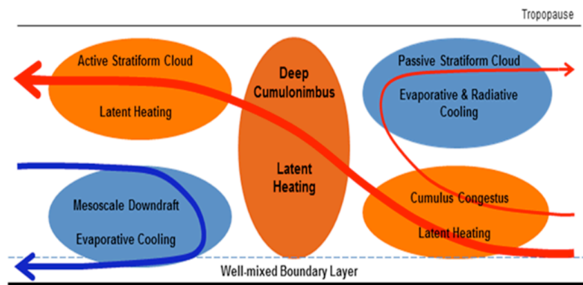
Figure 10. Multicloud parameterization adapted from Figure 6 of Khouider and Majda (2006). i) Brown hues represent warming tendencies by cumulus congestus, deep convection, and stratiform cloud. ii) Blue hues represent cooling by mesoscale downdrafts and radiation. The overlying curves show the 3-branch slantwise layer overturning in Figure 4 herein mapped onto the multicloud parameterization.
