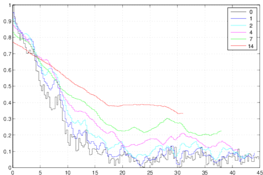
Figure 2. Correlation of a tornado environment index (TEI; Tippett et al. 2012) with CFSv2 forecasts during 2013 for averaging windows ranging from 6 hours to 14 days
