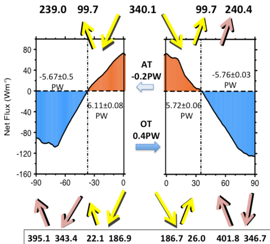
Figure 3. The annual-hemispheric mean energy balance of Earth. Unless specified otherwise, all TOA and surface numbers are in Wm^{-2} . Fluxes of sunlight entering and leaving the TOA and surface are in yellow and infrared fluxes are red (Stephens and L'Ecuyer, 2015). Our best estimate of the cross equatorial heat transport by atmosphere (AT) and oceans in PW (OT) are also given.
