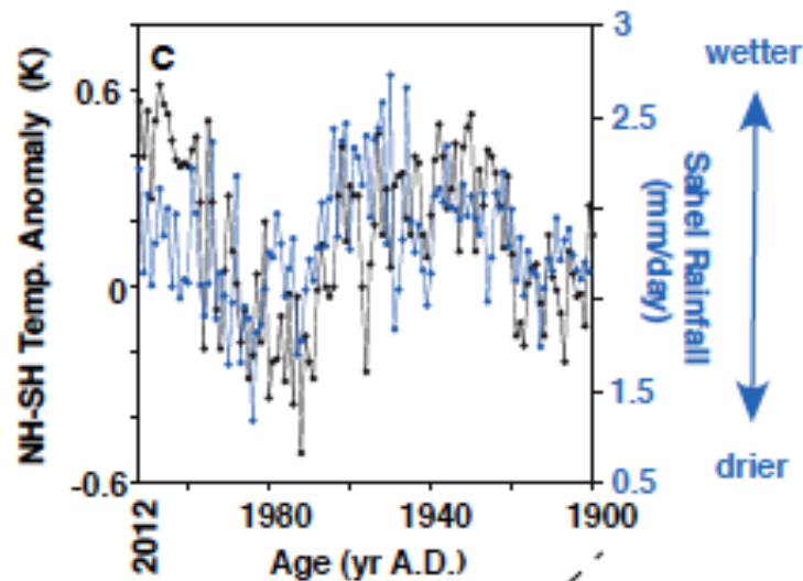
Figure 5. Temperature contrast between northern and southern hemisphere extra-tropics (poleward of 24°N/S) based on instrumental data (black), and average daily rainfall over the Sahel (12°-18°N, 20°W-35°E) during June-October based on land station data (blue). All temperatures and temperature contrasts are given as anomalies relative to the 1960-91 annual mean.
