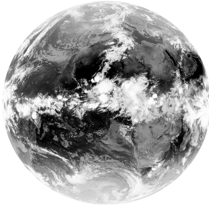
Figure 9. Multiscale organization of tropical convection
