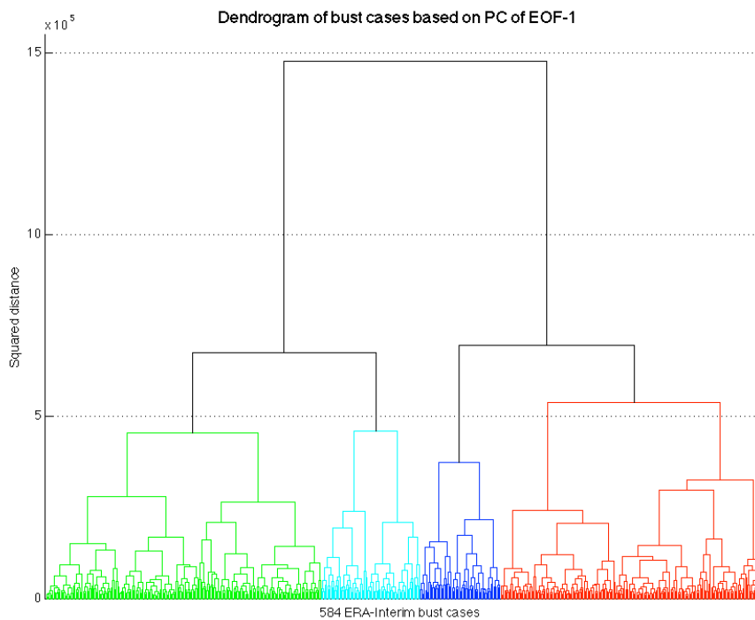
Figure 7. A dendrogram based a cluster analysis of the bust cases identified by Rodwell et al. (2013). The clustering was based the Principal Component Analysis scores of the first Emperical Orthogonal Function yielding different phenomena and large-scale wave patterns.
