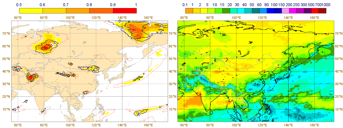
Figure 4. Left panel: ECMWF Extreme forecast index (EFI), shaded (see legend) and red contours (=0.3), and Shift of tails (SOT, black contours) for 24h precipitation, for a 72-96h lead, for a period ending 00UTC 25 February 2015. Right panel: 99th percentile of 24h precipitation for late February, computed from 20 years of re-forecasts. Note the large EFI and SOT values near the Pakistan-Afghanistan border warning of extreme weather in advance; the associated avalanches and flooding killed over 200 people. The right panel helps one to quantify ‘extreme’ in terms of actual precipitation; high EFI values near 60N/80E would very probably be associated with much smaller amounts than the high EFI values over Pakistan/Afghanistan.
