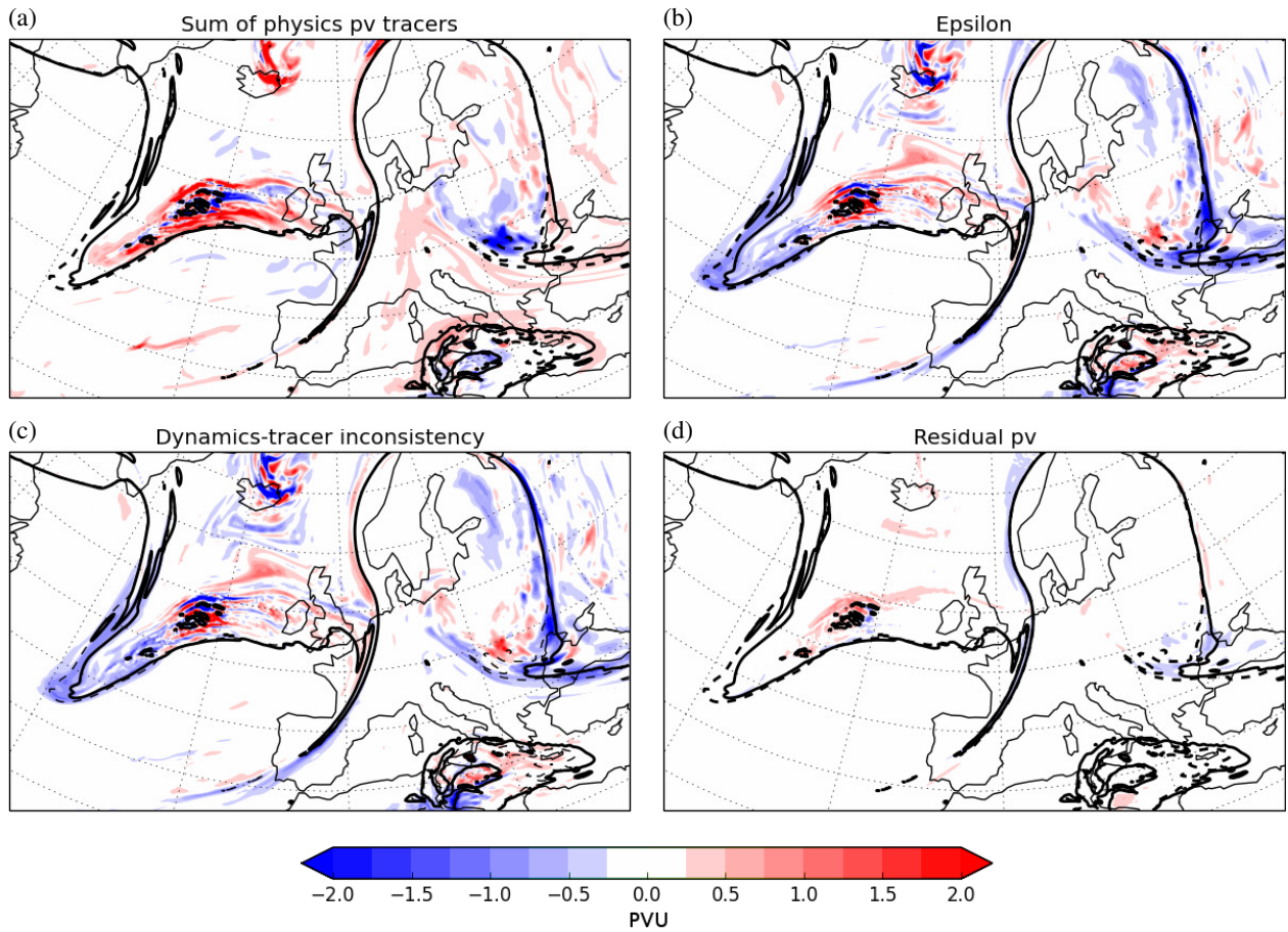
Figure 2. (a) The sum of the physics PV tracers ( \sum q_{physics} ). (b) \epsilon as defined by Eq. (18). (c) Dynamics-tracer inconsistency. (d) The residual in the PV budget ( \epsilon_r in Eq. (33)). All plots are linearly interpolated to the 320 K isentrope for a 36 h forecast. The thick black line in each plot is the 2 PVU line of the diagnosed PV and the dashed line is the 2 PVU line of the advection-only PV tracer
