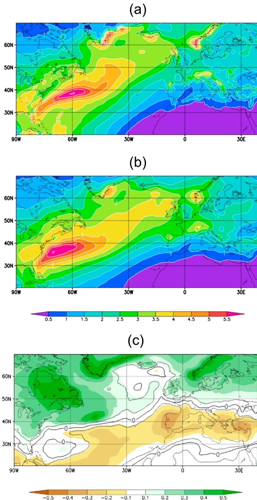
Figure 1. (a) ERA-Interim annual mean precipitation (in \text{mm d}^{-1} ). (b) Ensemble mean annual mean precipitation (in \text{mm d}^{-1} ) for 1979–2005. (c) Climate change signal (RCP8.5, 2071–2100 minus 1979–2005) of annual mean precipitation (in \text{mm d}^{-1} ). Statistically significant changes at 95% confidence level are delimited by dotted lines.
