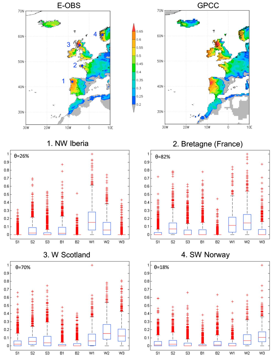
Figure 4. (top row) Fraction of explained variance of the monthly precipitation by the eight WT modes ((left) E-OBS data set, version 11.0, 0.25° grid; (right) GPCC, version 6, 0.5° grid), estimated by stepwise multivariate regressions, over the western European sector and for the period 1979–2014 (E-OBS) or 1979–2010 (GPCC). (middle and bottom rows) Boxplot charts of the daily precipitation totals (normalized to unit maximum) associated with each WT over the period of 1979–2014 and for the four outlined locations: 1—northwest Iberia; 2—Bretagne (France); 3—western Scotland, and 4—southwest Norway (see top left panel and text for geographical coordinates). Medians are horizontal lines, upper (lower) box limits are the 75th (25th) percentiles, upper (lower) whiskers limits are nonoutlier maxima (minima) and “plus” symbols are outliers (absolute distance to median > 1.5 \times interquartile range). The corresponding discriminatory powers ( \theta ) at each location are also outlined.
