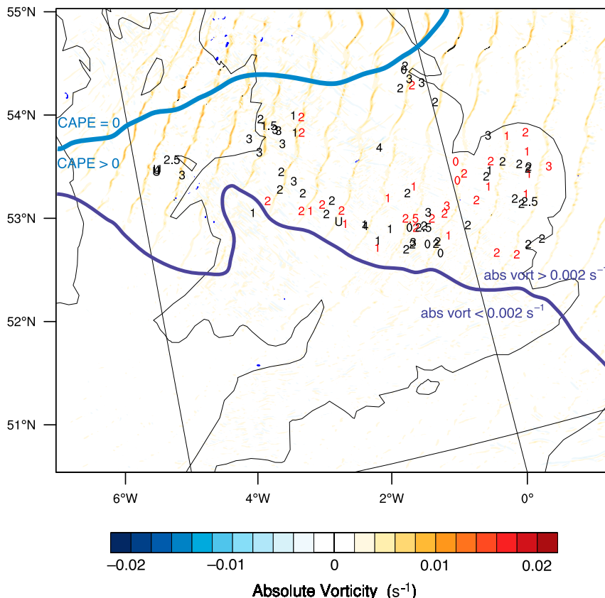
FIG. 22. Simulation of absolute vorticity at 500 m ASL ( s^{-1} ; colored according to scale) every 30 min from 0900 to 1800 UTC on the domain with 1-km horizontal grid spacing. Purple lines separate approximate areas with simulated absolute vorticity less than 0.002 s^{-1} on the 1-km domain during the time of frontal passage. Blue lines separate approximate areas with simulated positive CAPE during the time of frontal passage. Locations of reports that appear to be located over water are a result of a coarse representation of geography. Locations of the 90 tornado reports from the TORRO database for 23 Nov 1981. Numbers represent their strength on the T scale. Reports verified by TORRO (58) are classified as definite and plotted in black. Reports that have not been verified (32) are classified as probable and are plotted in red.
