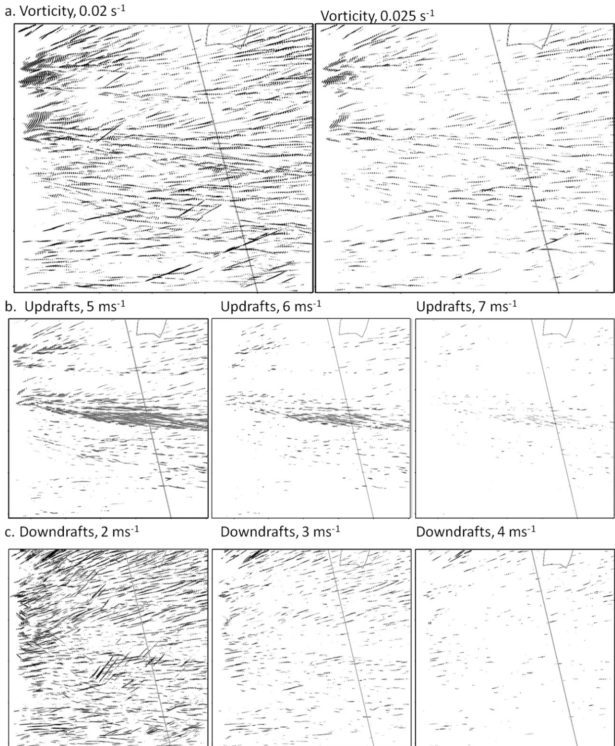
FIG. 20. Tracks of (a) 500-m absolute vorticity ( 0.02 and 0.025 \text{ s}^{-1} ), (b) 500-m updrafts ( 5 , 6 , and 7 \text{ ms}^{-1} ), and (c) 500-m downdrafts ( 2 , 3 , and 4 \text{ ms}^{-1} ) plotted every minute from 1300 to 1600 UTC in the domain with 200-m horizontal grid spacing.
