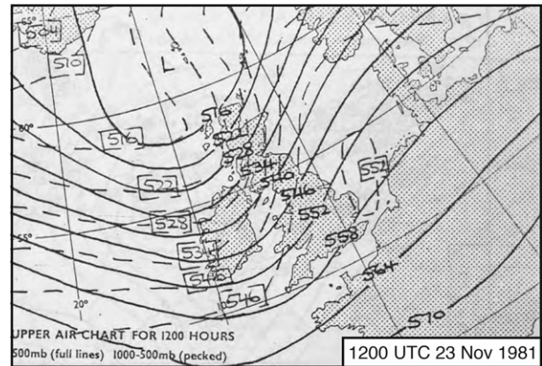
FIG. 4. Excerpt from Met Office Daily Weather Summary 500-hPa chart at 1200 UTC 23 Nov 1981. Plotted are 500-hPa geopotential height (solid lines every 6 dam) and 1000–500-hPa thickness (dashed lines every 6 dam). (Crown copyright.)
