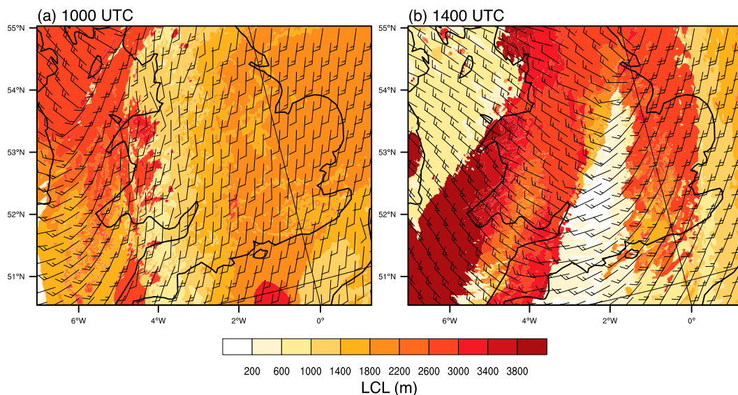
FIG. 14. As in Fig. 10, but for simulation of LCL (m; colored according to scale) and surface winds.
