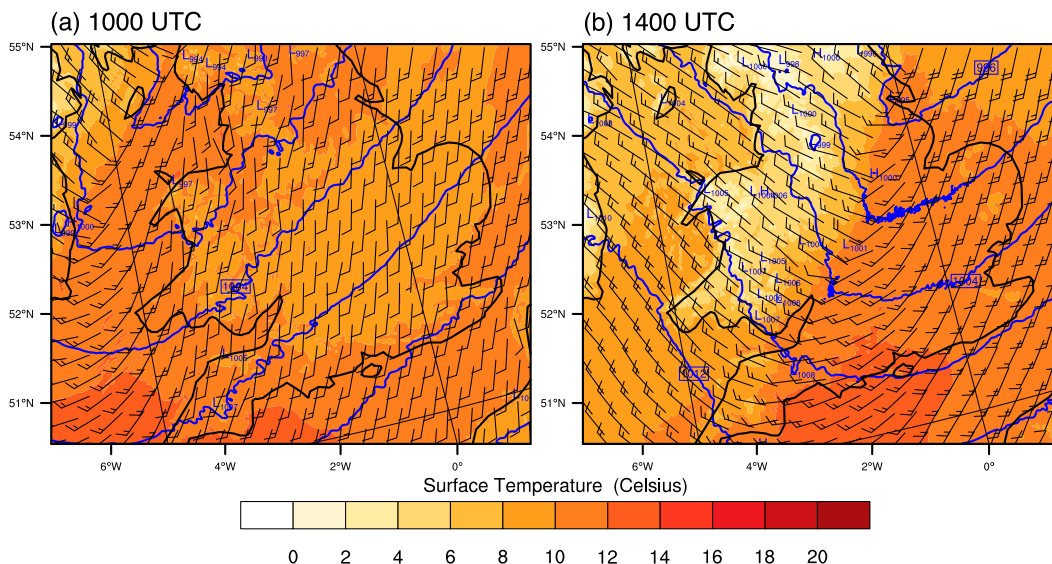
FIG. 10. Simulation of sea level pressure (hPa; blue lines), surface temperature ( ^{\circ}\text{C} ; colored according to scale), and surface winds (pennant; full barb, and half barb denote 25 , 5 , and 2.5 \text{m s}^{-1} , respectively; separation between displayed wind vectors is 30 km) on the domain with 1 -km horizontal grid spacing at (a) 1000 and (b) 1400 UTC 23 Nov 1981 .
