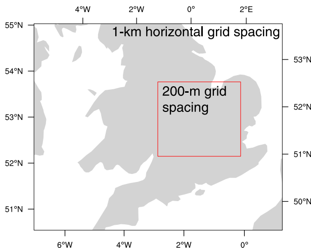
FIG. 9. The two innermost domains used in this simulation.
