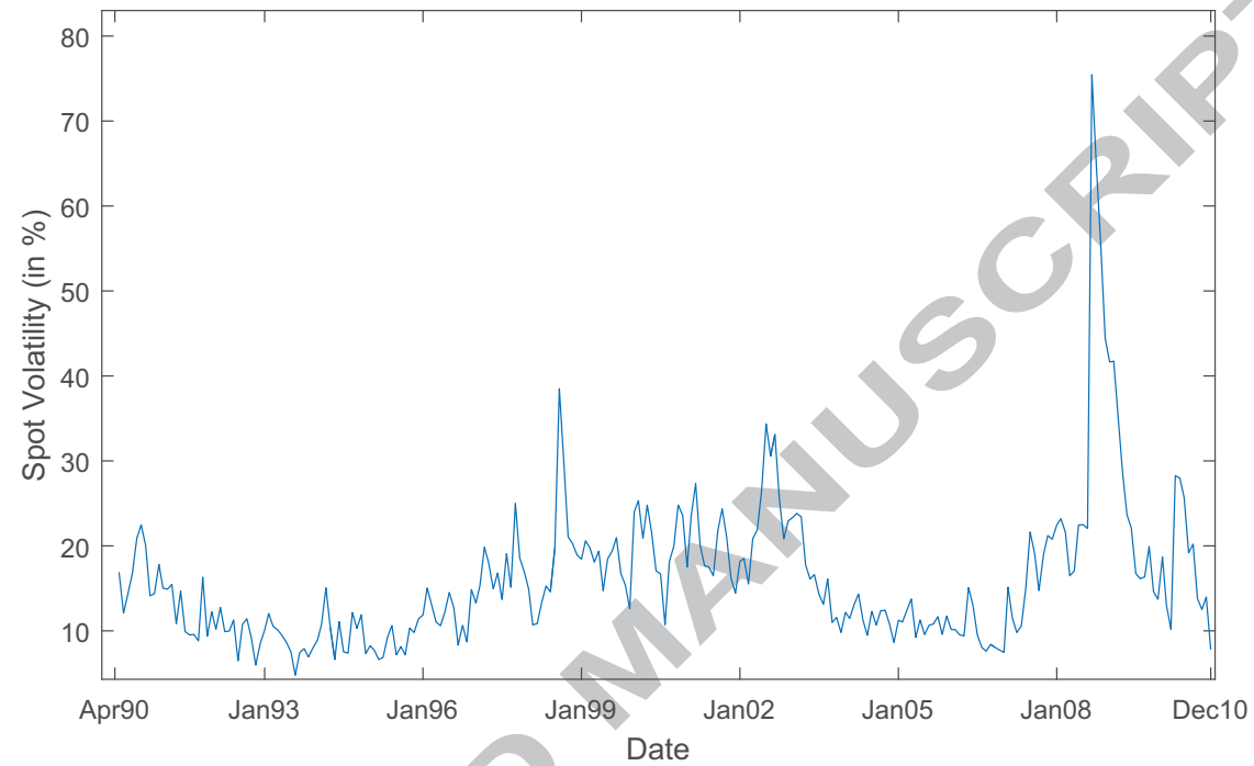
Figure 1: Latent Volatility
